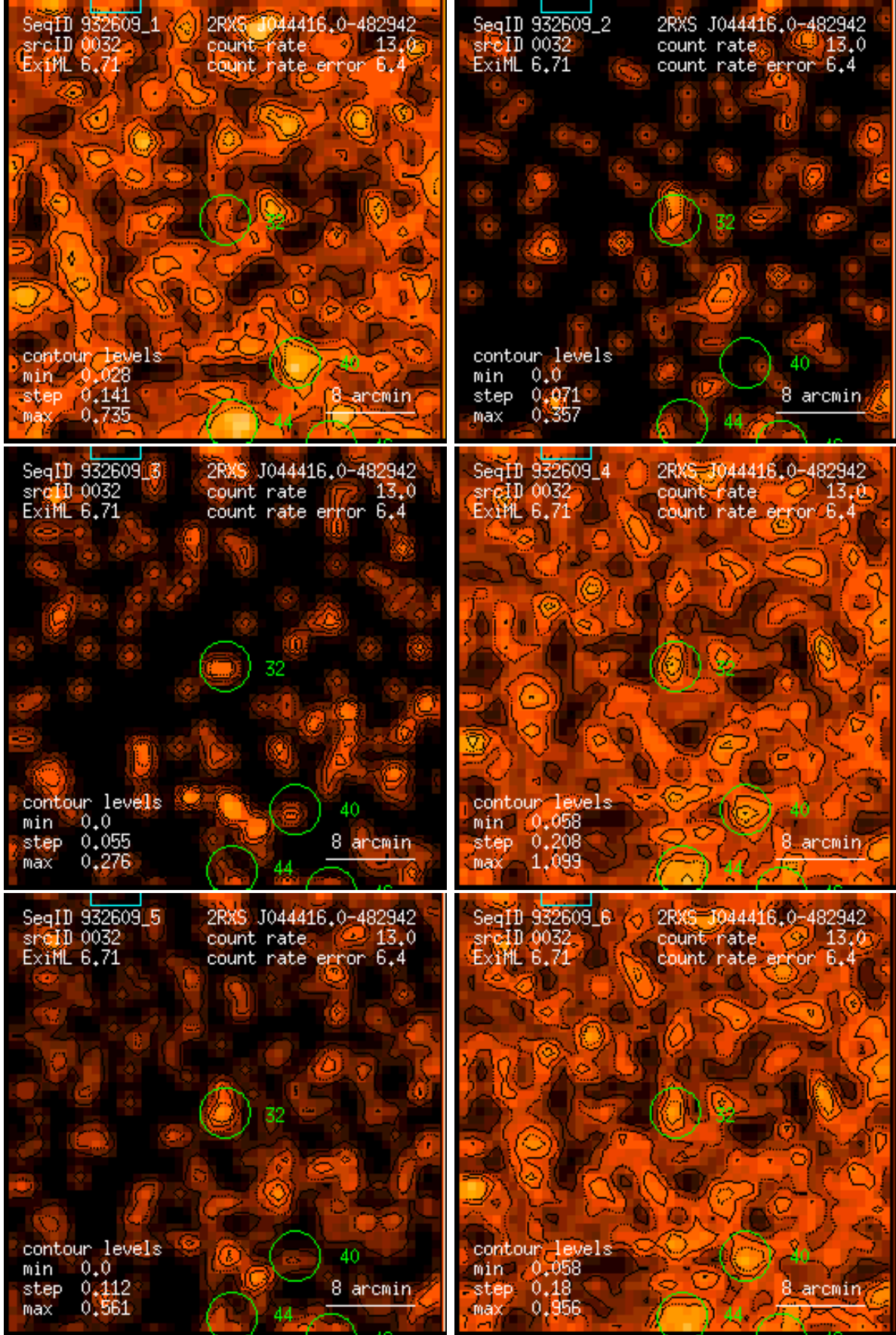
Figure 32: RASS 932609: detection 0032: band rate images, Gaussian filter: (1) PSPC channels 11 – 41, (2) 52 – 90, (3) 91 – 201, (4) 11 – 235, (5) 52 – 201, (6) 11 – 201. Broad band rates in counts/ks. Band rate contour levels in counts/ks/arcmin 2 .
