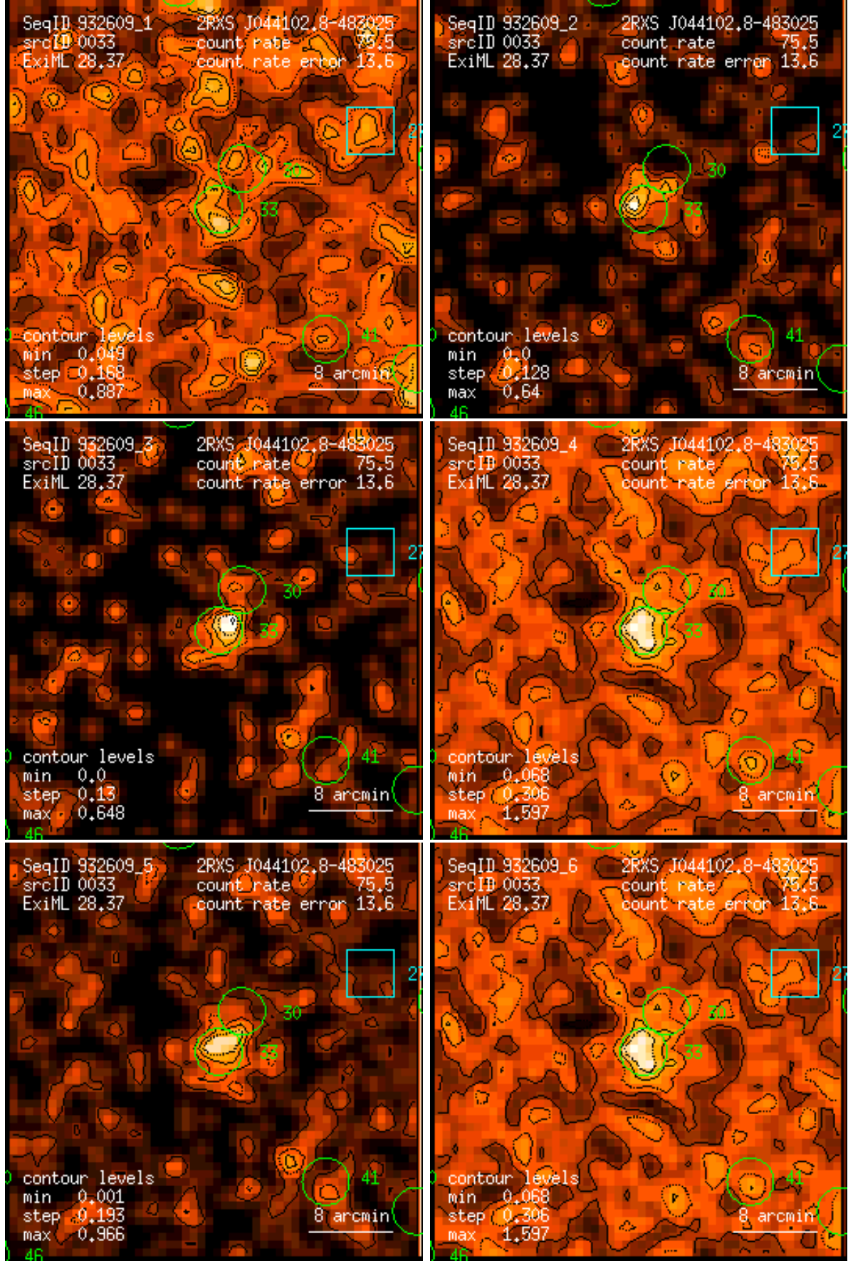
Figure 33: RASS 932609: detection 0033: band rate images, Gaussian filter: (1) PSPC channels 11 – 41, (2) 52 – 90, (3) 91 – 201, (4) 11 – 235, (5) 52 – 201, (6) 11 – 201. Broad band rates in counts/ks. Band rate contour levels in counts/ks/arcmin 2 .
