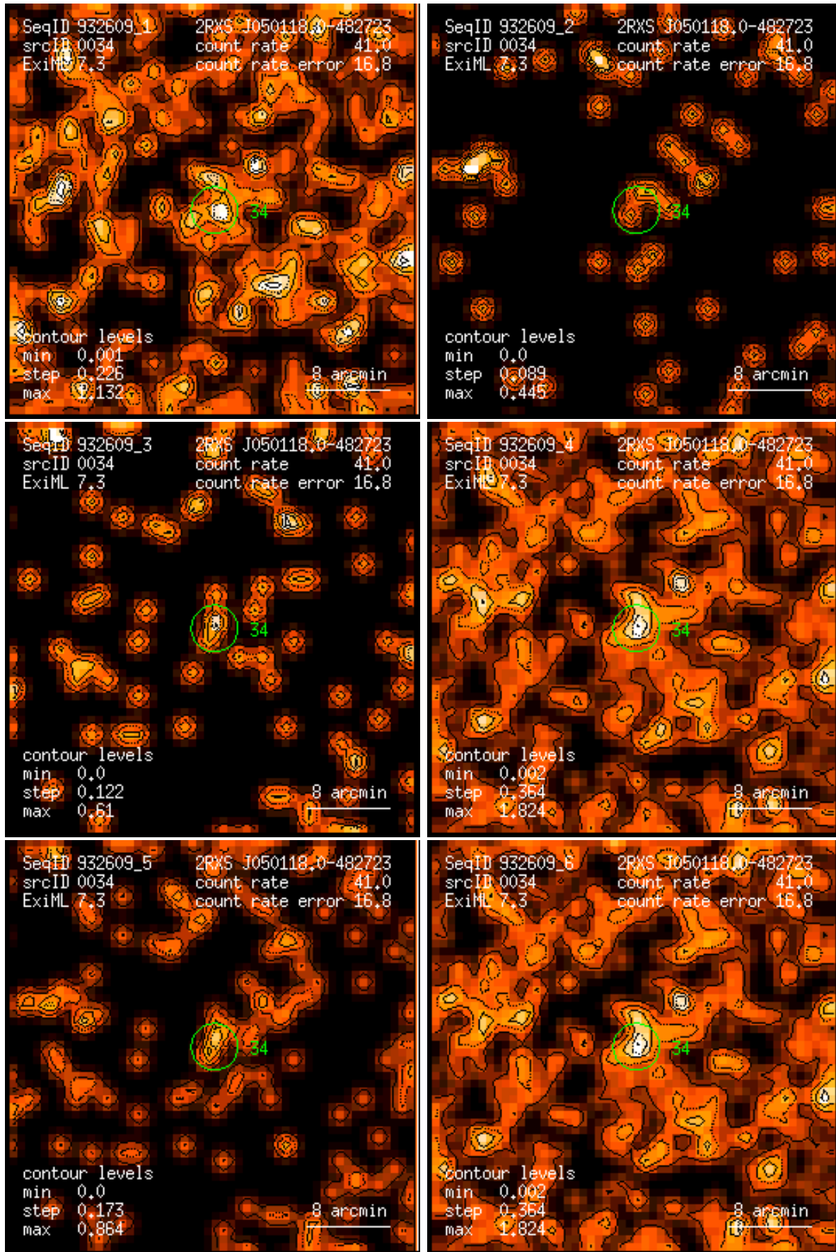
Figure 34: RASS 932609: detection 0034: band rate images, Gaussian filter: (1) PSPC channels 11 – 41, (2) 52 – 90, (3) 91 – 201, (4) 11 – 235, (5) 52 – 201, (6) 11 – 201. Broad band rates in counts/ks. Band rate contour levels in counts/ks/arcmin 2 .
