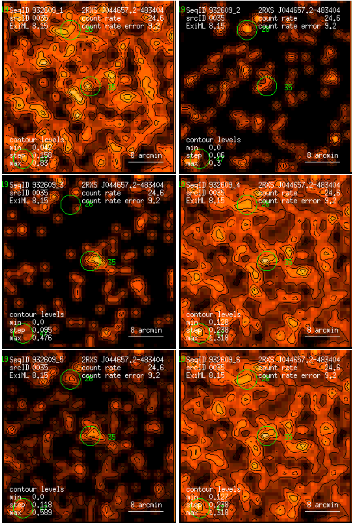
Figure 35: RASS 932609: detection 0035: band rate images, Gaussian filter: (1) PSPC channels 11 – 41, (2) 52 – 90, (3) 91 – 201, (4) 11 – 235, (5) 52 – 201, (6) 11 – 201. Broad band rates in counts/ks. Band rate contour levels in counts/ks/arcmin 2 .
