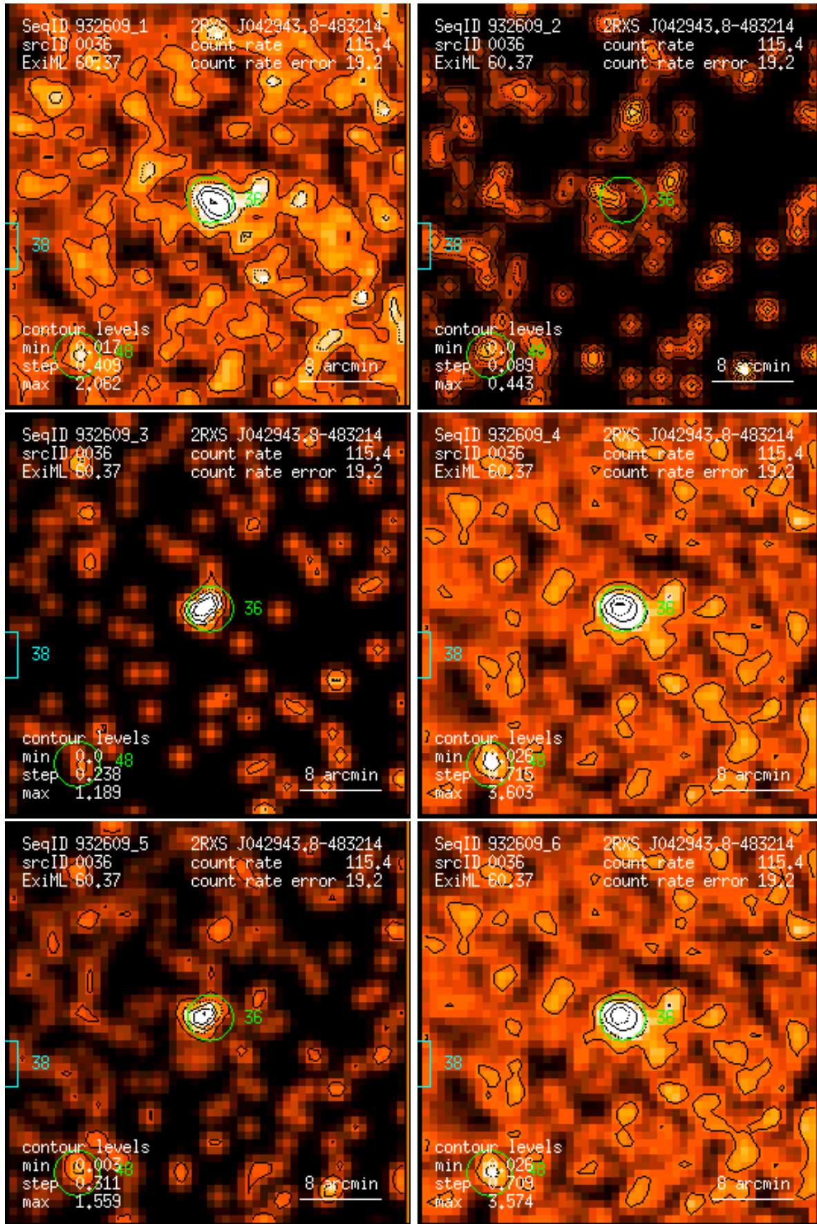
Figure 36: RASS 932609: detection 0036: band rate images, Gaussian filter: (1) PSPC channels 11 – 41, (2) 52 – 90, (3) 91 – 201, (4) 11 – 235, (5) 52 – 201, (6) 11 – 201. Broad band rates in counts/ks. Band rate contour levels in counts/ks/arcmin 2 .
