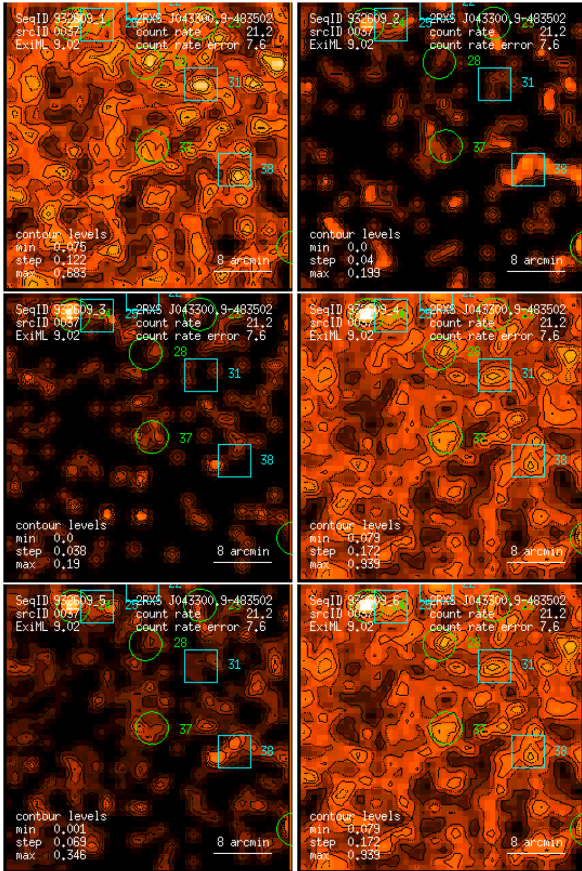
Figure 37: RASS 932609: detection 0037: band rate images, Gaussian filter: (1) PSPC channels 11 – 41, (2) 52 – 90, (3) 91 – 201, (4) 11 – 235, (5) 52 – 201, (6) 11 – 201. Broad band rates in counts/ks. Band rate contour levels in counts/ks/arcmin 2 .
