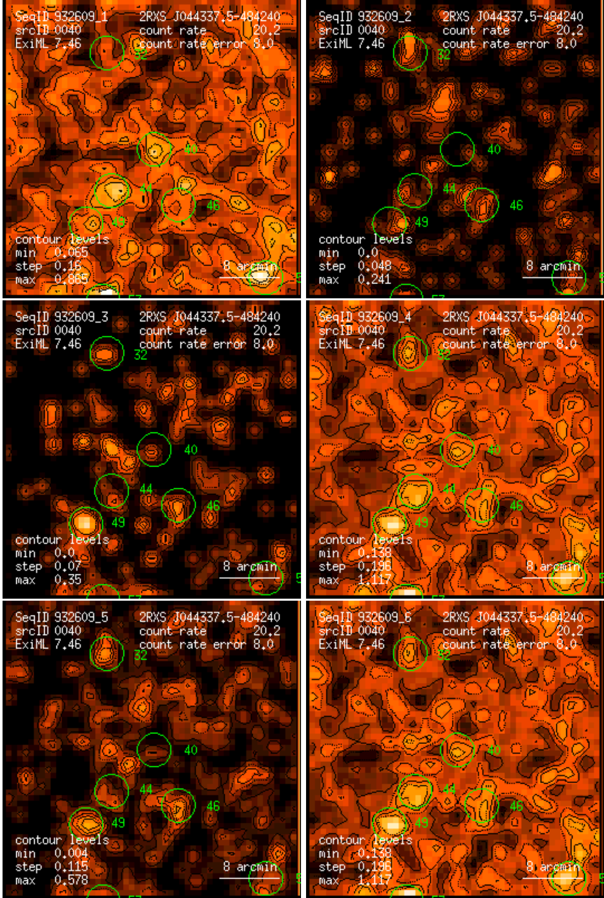
Figure 40: RASS 932609: detection 0040: band rate images, Gaussian filter: (1) PSPC channels 11 – 41, (2) 52 – 90, (3) 91 – 201, (4) 11 – 235, (5) 52 – 201, (6) 11 – 201. Broad band rates in counts/ks. Band rate contour levels in counts/ks/arcmin 2 .
