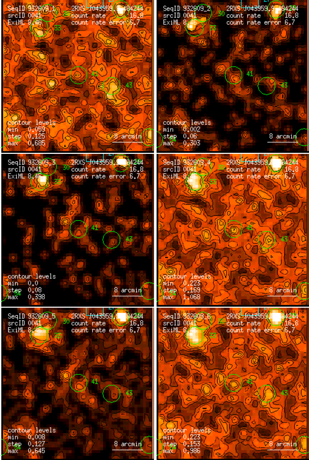
Figure 41: RASS 932609: detection 0041: band rate images, Gaussian filter: (1) PSPC channels 11 – 41, (2) 52 – 90, (3) 91 – 201, (4) 11 – 235, (5) 52 – 201, (6) 11 – 201. Broad band rates in counts/ks. Band rate contour levels in counts/ks/arcmin 2 .
