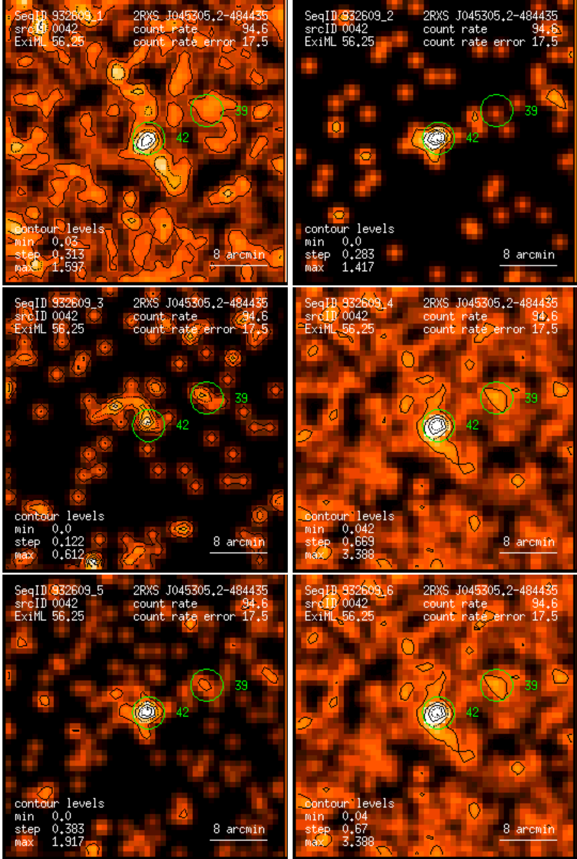
Figure 42: RASS 932609: detection 0042: band rate images, Gaussian filter: (1) PSPC channels 11 – 41, (2) 52 – 90, (3) 91 – 201, (4) 11 – 235, (5) 52 – 201, (6) 11 – 201. Broad band rates in counts/ks. Band rate contour levels in counts/ks/arcmin 2 .
