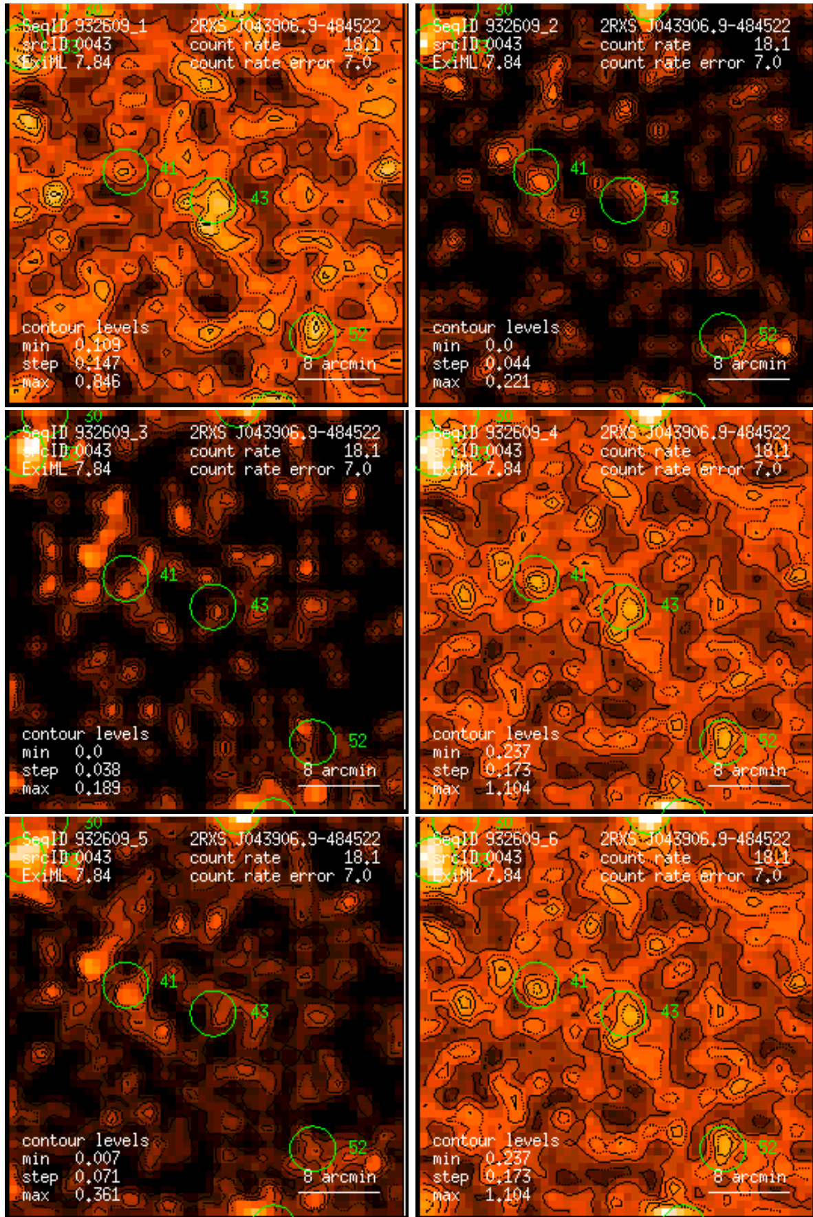
Figure 43: RASS 932609: detection 0043: band rate images, Gaussian filter: (1) PSPC channels 11 – 41, (2) 52 – 90, (3) 91 – 201, (4) 11 – 235, (5) 52 – 201, (6) 11 – 201. Broad band rates in counts/ks. Band rate contour levels in counts/ks/arcmin 2 .
