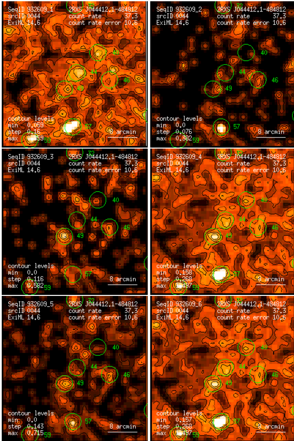
Figure 44: RASS 932609: detection 0044: band rate images, Gaussian filter: (1) PSPC channels 11 – 41, (2) 52 – 90, (3) 91 – 201, (4) 11 – 235, (5) 52 – 201, (6) 11 – 201. Broad band rates in counts/ks. Band rate contour levels in counts/ks/arcmin 2 .
