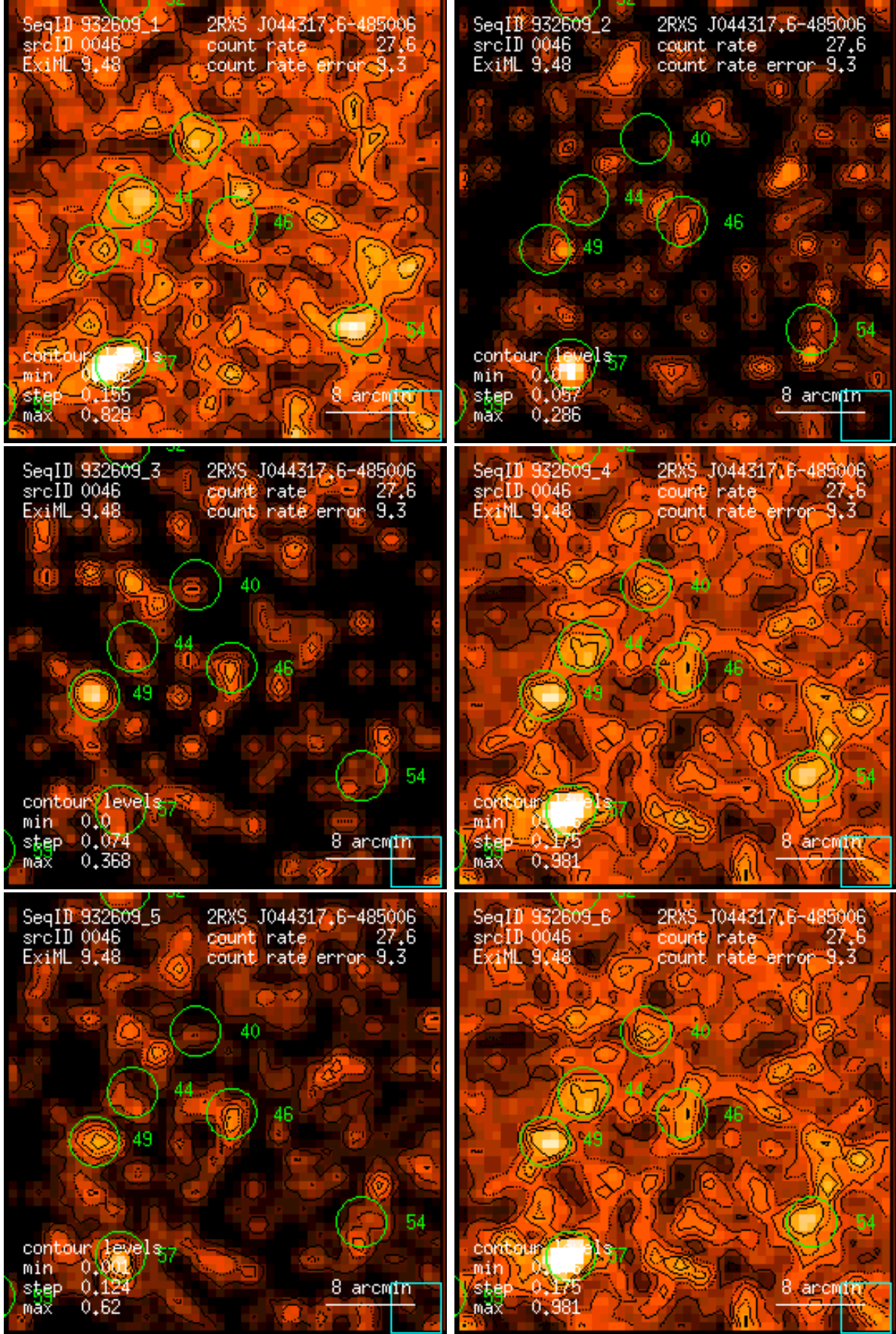
Figure 46: RASS 932609: detection 0046: band rate images, Gaussian filter: (1) PSPC channels 11 – 41, (2) 52 – 90, (3) 91 – 201, (4) 11 – 235, (5) 52 – 201, (6) 11 – 201. Broad band rates in counts/ks. Band rate contour levels in counts/ks/arcmin 2 .
