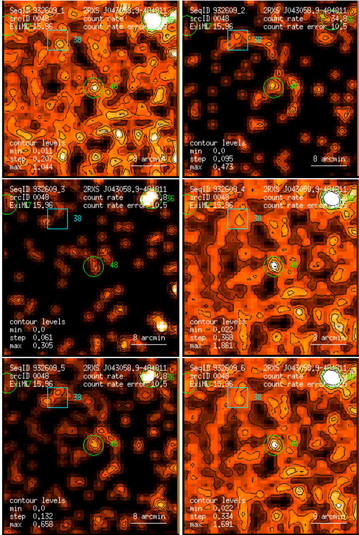
Figure 48: RASS 932609: detection 0048: band rate images, Gaussian filter: (1) PSPC channels 11 – 41, (2) 52 – 90, (3) 91 – 201, (4) 11 – 235, (5) 52 – 201, (6) 11 – 201. Broad band rates in counts/ks. Band rate contour levels in counts/ks/arcmin 2 .
