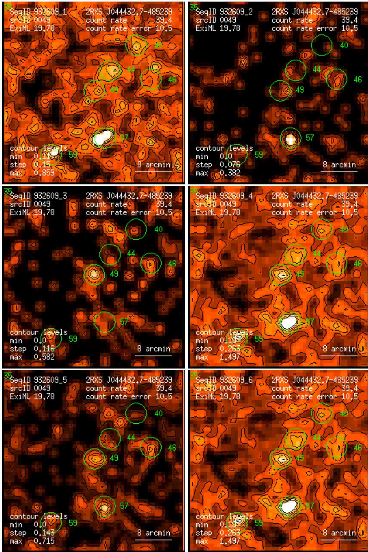
Figure 49: RASS 932609: detection 0049: band rate images, Gaussian filter: (1) PSPC channels 11 – 41, (2) 52 – 90, (3) 91 – 201, (4) 11 – 235, (5) 52 – 201, (6) 11 – 201. Broad band rates in counts/ks. Band rate contour levels in counts/ks/arcmin 2 .
