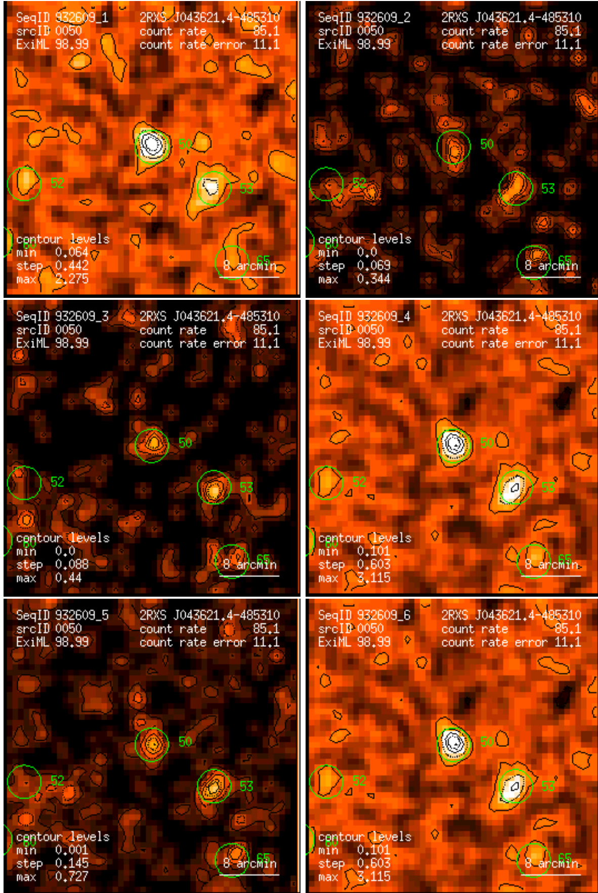
Figure 50: RASS 932609: detection 0050: band rate images, Gaussian filter: (1) PSPC channels 11 – 41, (2) 52 – 90, (3) 91 – 201, (4) 11 – 235, (5) 52 – 201, (6) 11 – 201. Broad band rates in counts/ks. Band rate contour levels in counts/ks/arcmin 2 .
