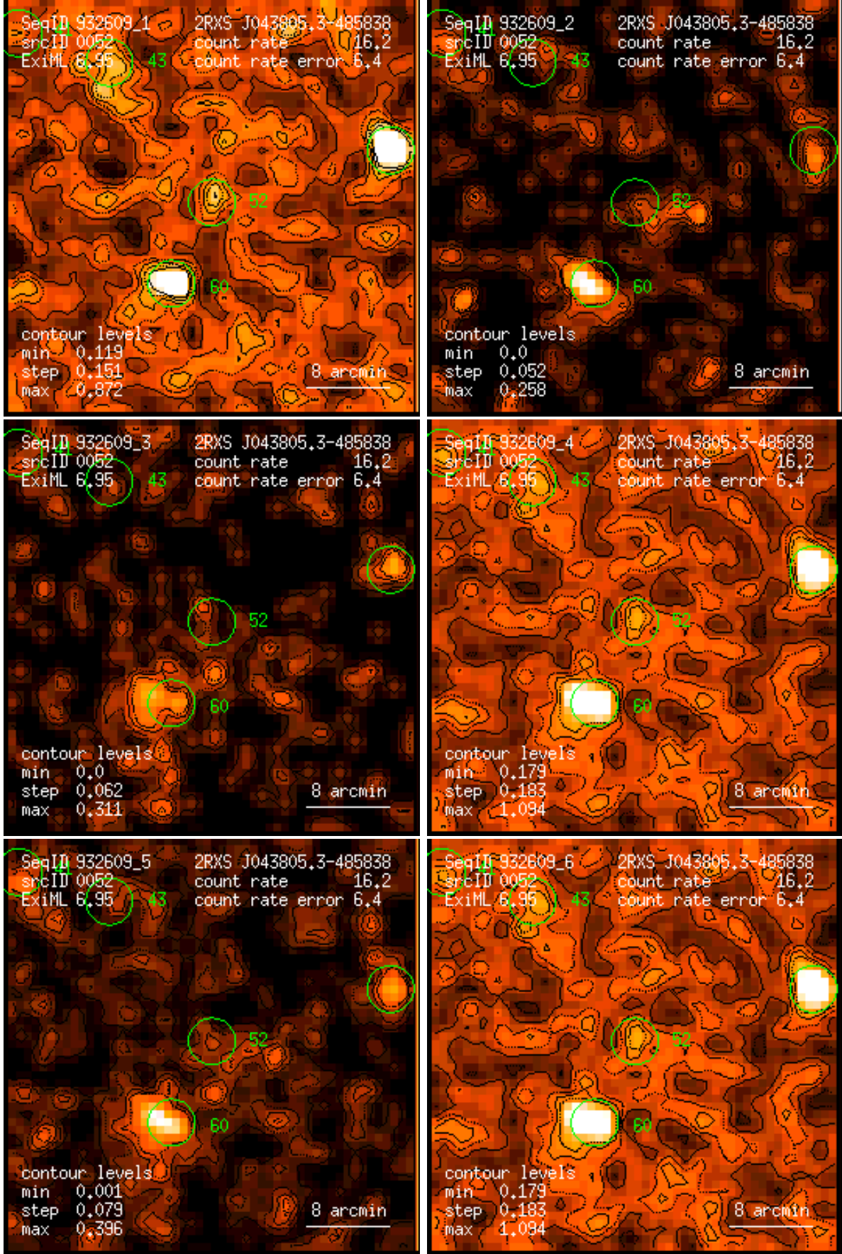
Figure 52: RASS 932609: detection 0052: band rate images, Gaussian filter: (1) PSPC channels 11 – 41, (2) 52 – 90, (3) 91 – 201, (4) 11 – 235, (5) 52 – 201, (6) 11 – 201. Broad band rates in counts/ks. Band rate contour levels in counts/ks/arcmin 2 .
