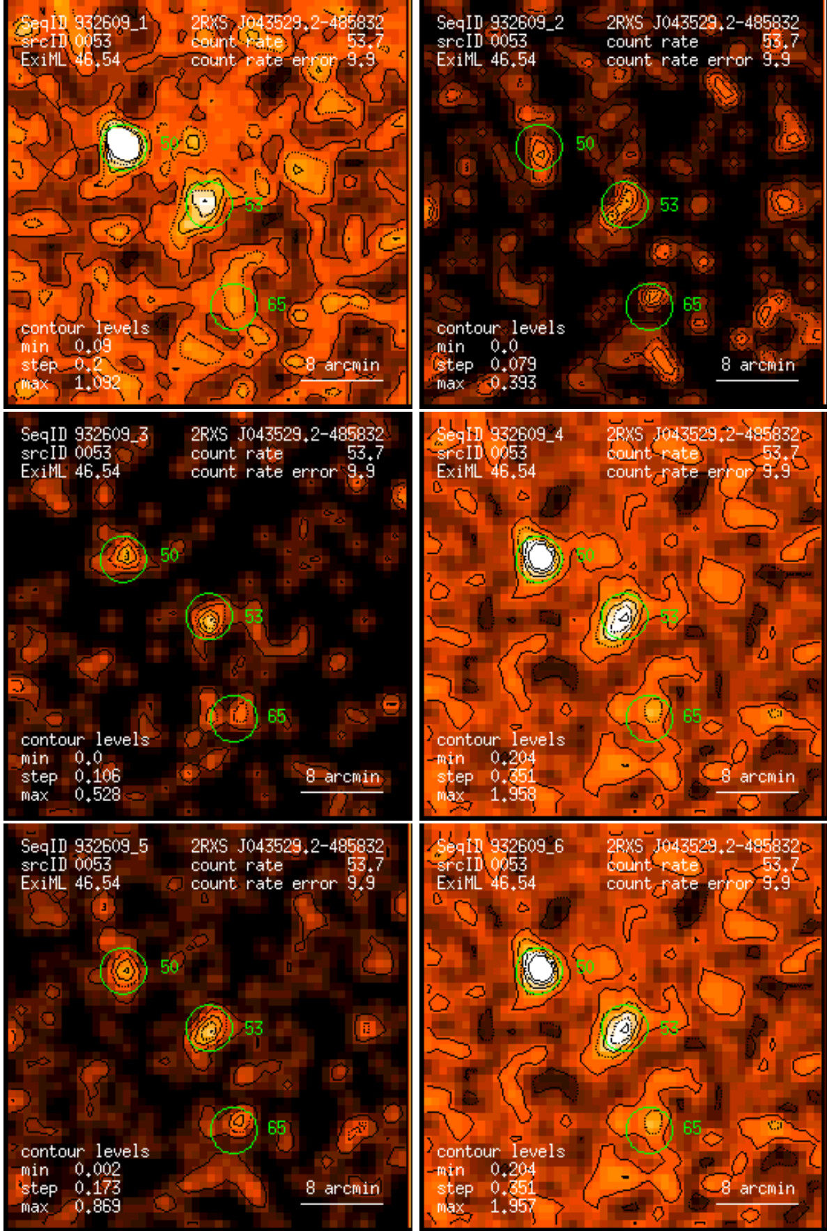
Figure 53: RASS 932609: detection 0053: band rate images, Gaussian filter: (1) PSPC channels 11 – 41, (2) 52 – 90, (3) 91 – 201, (4) 11 – 235, (5) 52 – 201, (6) 11 – 201. Broad band rates in counts/ks. Band rate contour levels in counts/ks/arcmin 2 .
