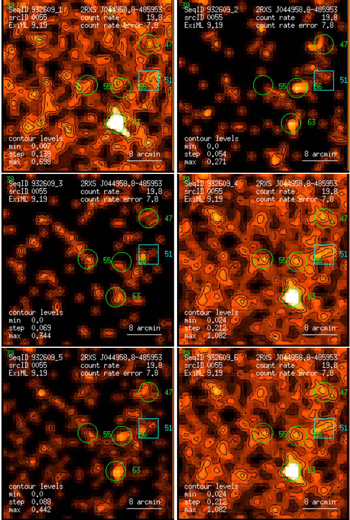
Figure 55: RASS 932609: detection 0055: band rate images, Gaussian filter: (1) PSPC channels 11 – 41, (2) 52 – 90, (3) 91 – 201, (4) 11 – 235, (5) 52 – 201, (6) 11 – 201. Broad band rates in counts/ks. Band rate contour levels in counts/ks/arcmin 2 .
