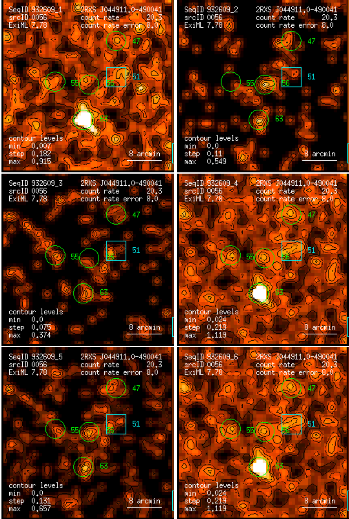
Figure 56: RASS 932609: detection 0056: band rate images, Gaussian filter: (1) PSPC channels 11 – 41, (2) 52 – 90, (3) 91 – 201, (4) 11 – 235, (5) 52 – 201, (6) 11 – 201. Broad band rates in counts/ks. Band rate contour levels in counts/ks/arcmin 2 .
