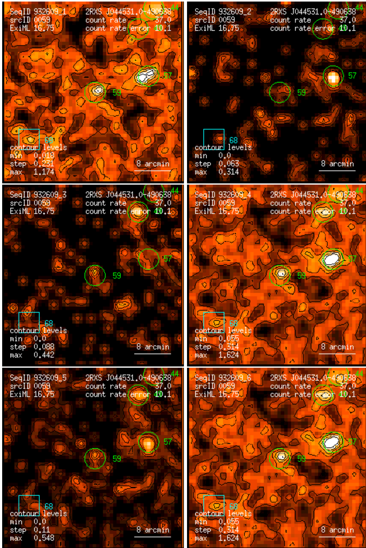
Figure 59: RASS 932609: detection 0059: band rate images, Gaussian filter: (1) PSPC channels 11 – 41, (2) 52 – 90, (3) 91 – 201, (4) 11 – 235, (5) 52 – 201, (6) 11 – 201. Broad band rates in counts/ks. Band rate contour levels in counts/ks/arcmin 2 .
