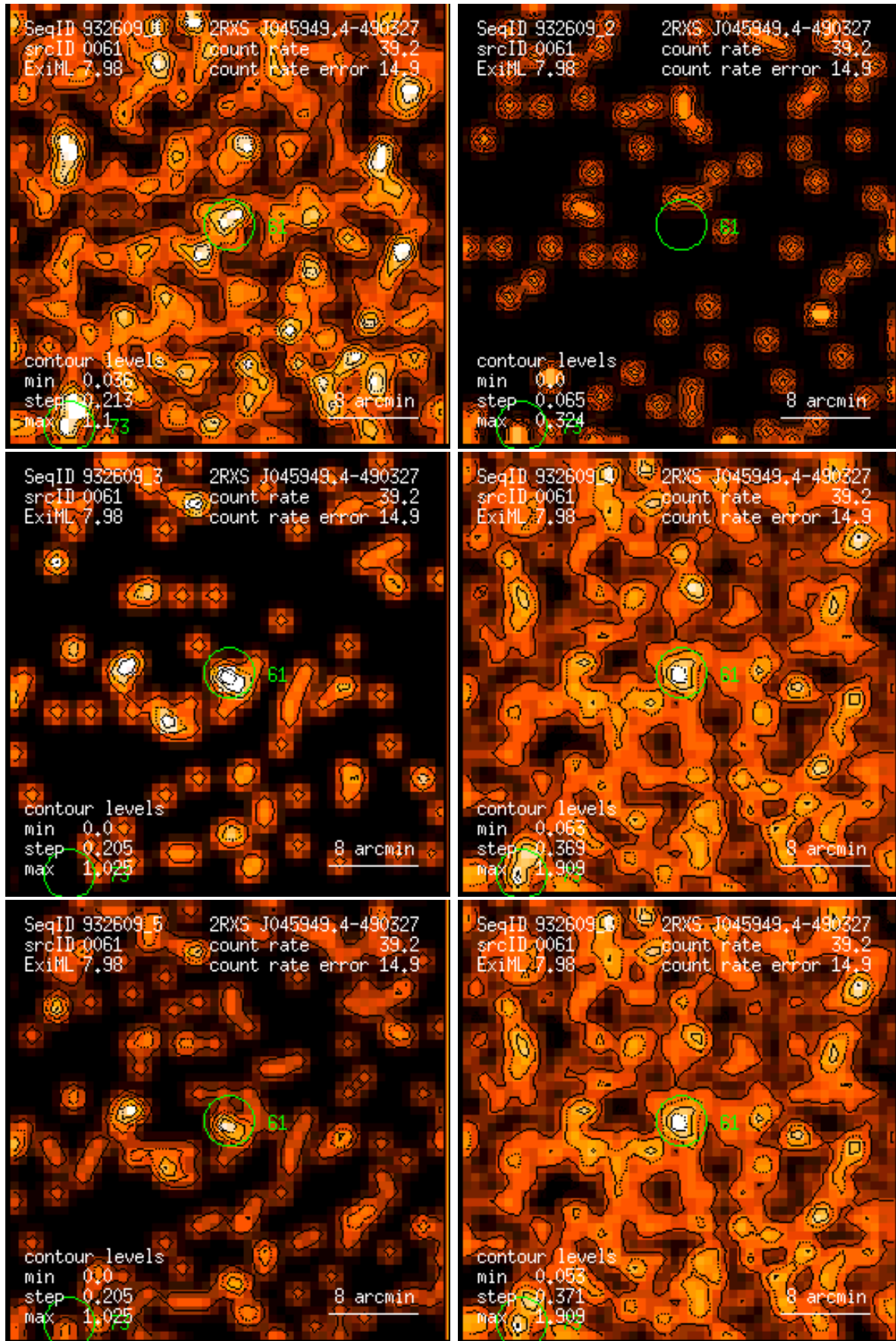
Figure 61: RASS 932609: detection 0061: band rate images, Gaussian filter: (1) PSPC channels 11 – 41, (2) 52 – 90, (3) 91 – 201, (4) 11 – 235, (5) 52 – 201, (6) 11 – 201. Broad band rates in counts/ks. Band rate contour levels in counts/ks/arcmin 2 .
