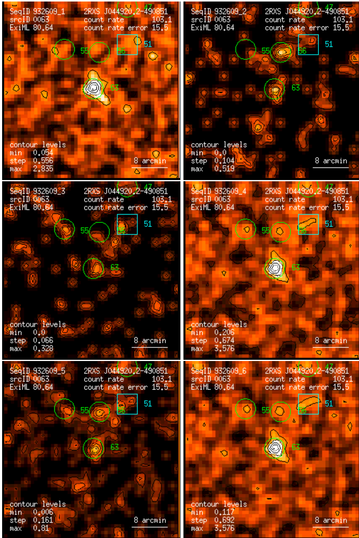
Figure 63: RASS 932609: detection 0063: band rate images, Gaussian filter: (1) PSPC channels 11 – 41, (2) 52 – 90, (3) 91 – 201, (4) 11 – 235, (5) 52 – 201, (6) 11 – 201. Broad band rates in counts/ks. Band rate contour levels in counts/ks/arcmin 2 .
