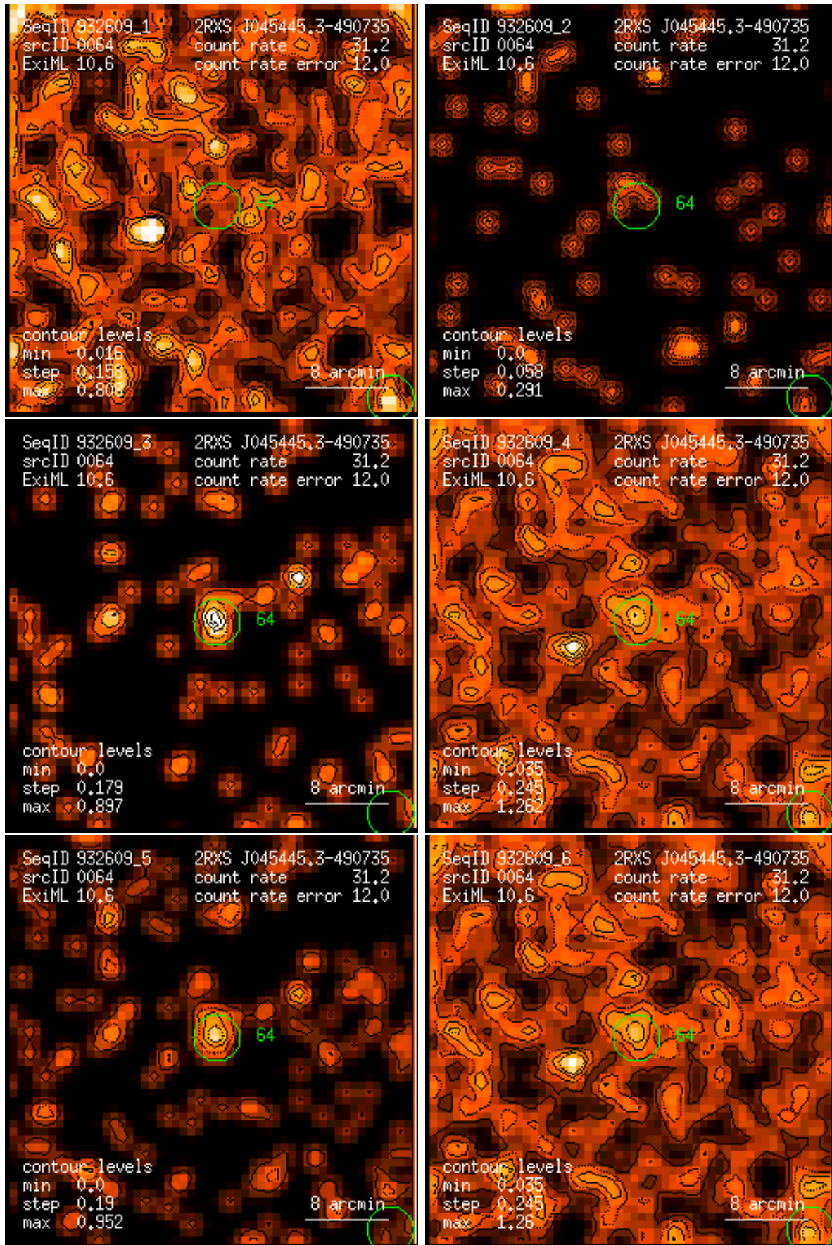
Figure 64: RASS 932609: detection 0064: band rate images, Gaussian filter: (1) PSPC channels 11 – 41, (2) 52 – 90, (3) 91 – 201, (4) 11 – 235, (5) 52 – 201, (6) 11 – 201. Broad band rates in counts/ks. Band rate contour levels in counts/ks/arcmin 2 .
