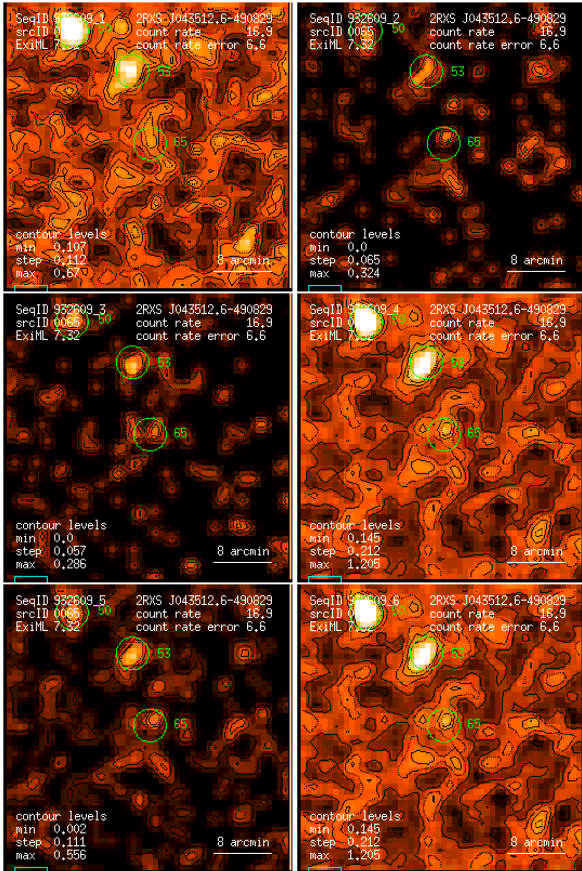
Figure 65: RASS 932609: detection 0065: band rate images, Gaussian filter: (1) PSPC channels 11 – 41, (2) 52 – 90, (3) 91 – 201, (4) 11 – 235, (5) 52 – 201, (6) 11 – 201. Broad band rates in counts/ks. Band rate contour levels in counts/ks/arcmin 2 .
