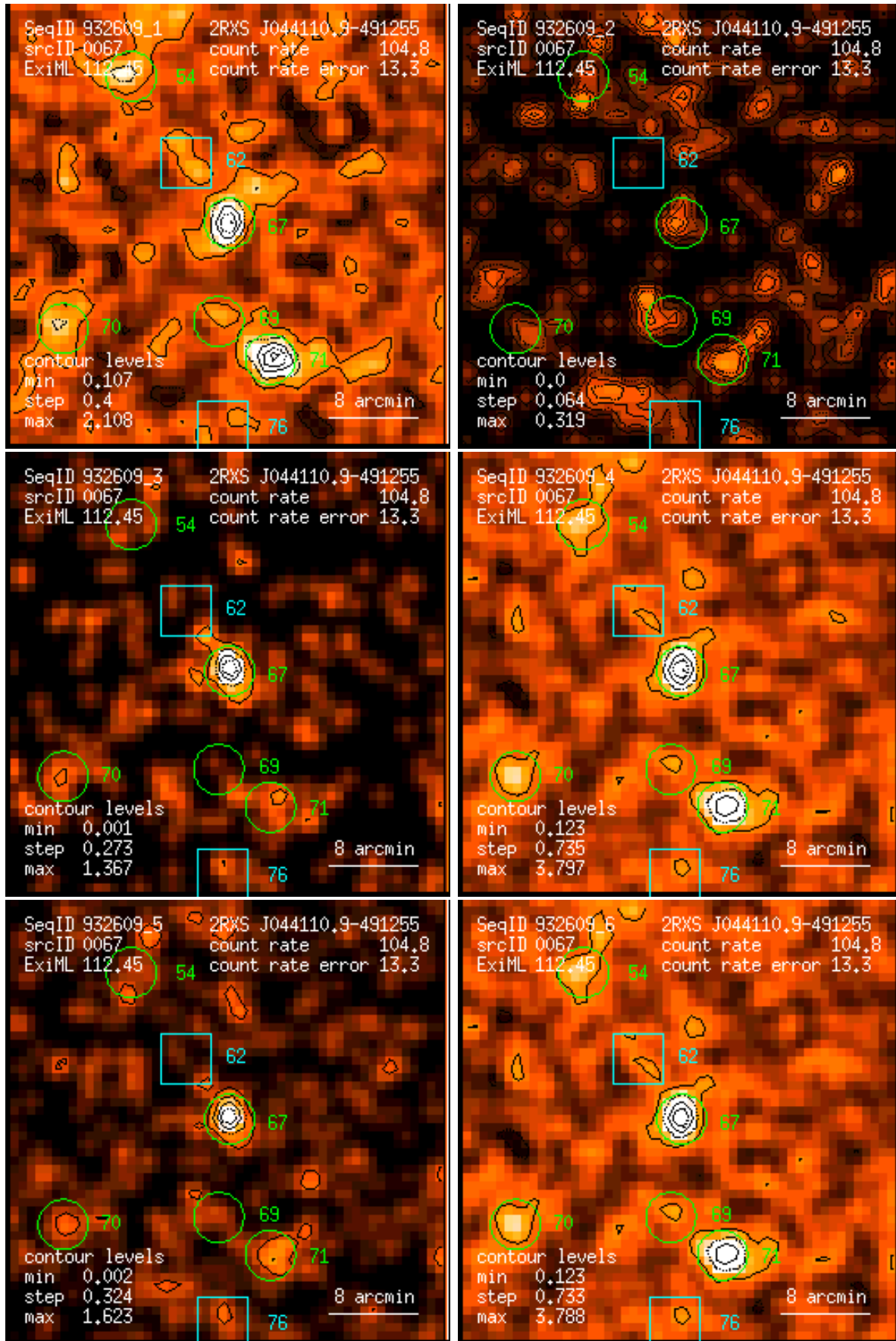
Figure 67: RASS 932609: detection 0067: band rate images, Gaussian filter: (1) PSPC channels 11 – 41, (2) 52 – 90, (3) 91 – 201, (4) 11 – 235, (5) 52 – 201, (6) 11 – 201. Broad band rates in counts/ks. Band rate contour levels in counts/ks/arcmin 2 .
