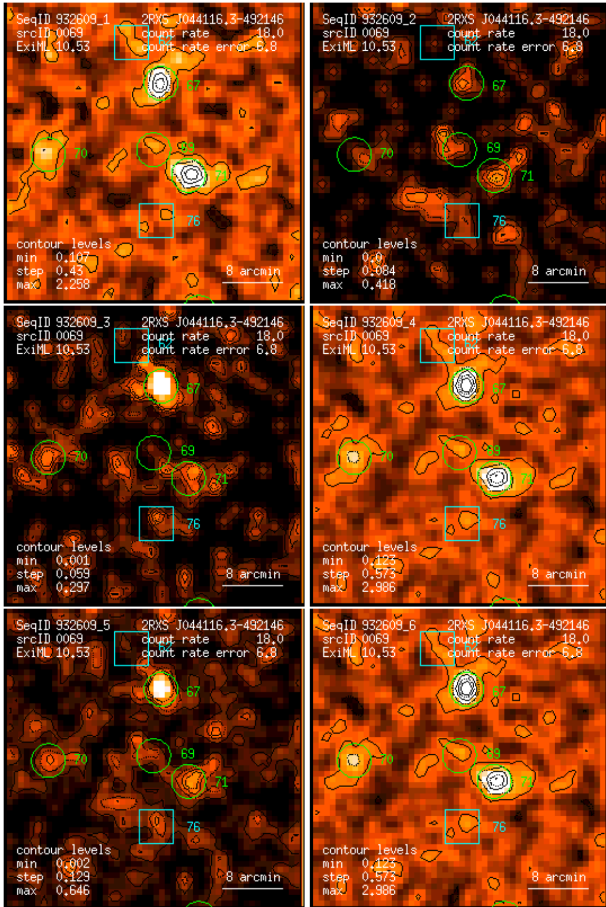
Figure 69: RASS 932609: detection 0069: band rate images, Gaussian filter: (1) PSPC channels 11 – 41, (2) 52 – 90, (3) 91 – 201, (4) 11 – 235, (5) 52 – 201, (6) 11 – 201. Broad band rates in counts/ks. Band rate contour levels in counts/ks/arcmin 2 .
