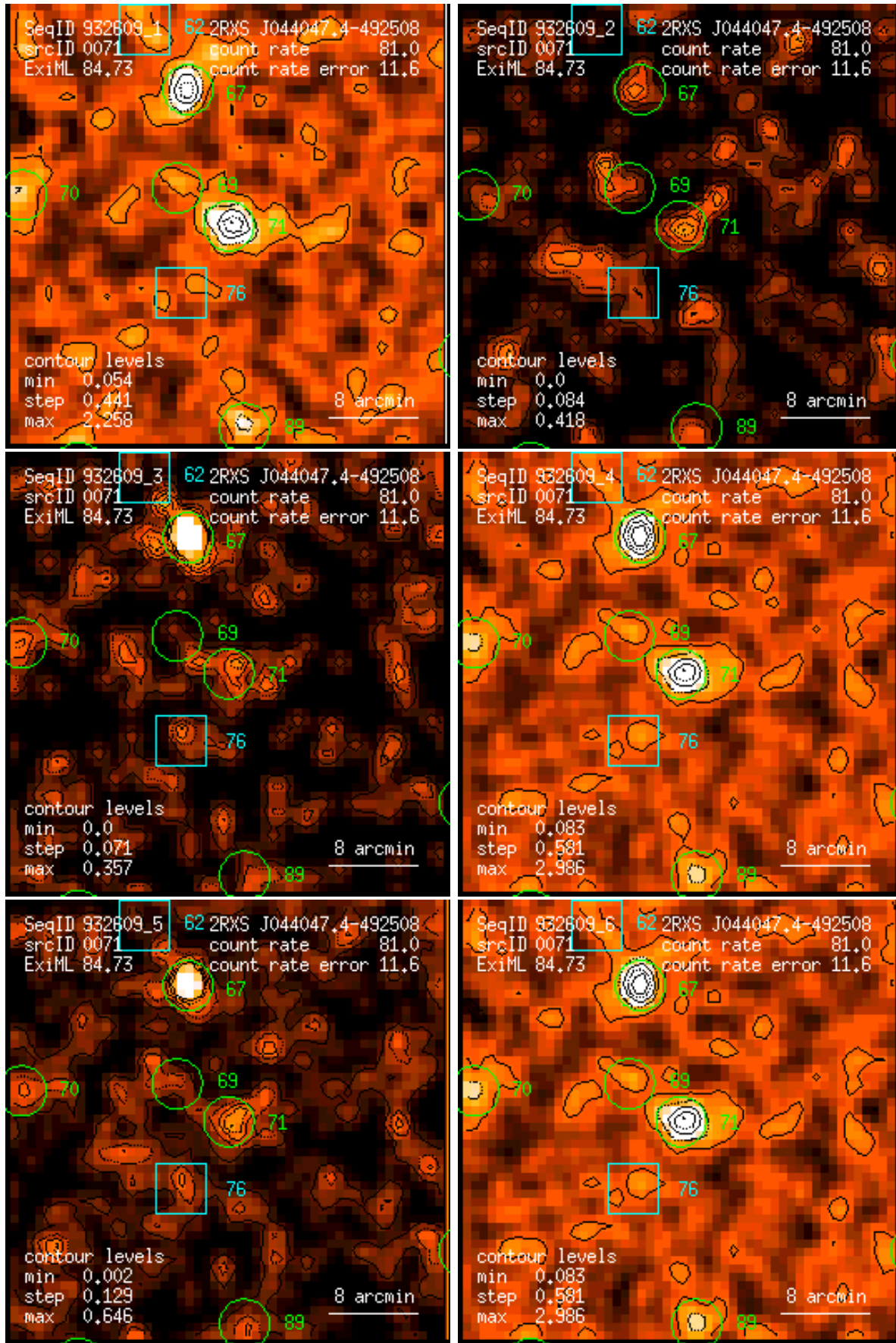
Figure 71: RASS 932609: detection 0071: band rate images, Gaussian filter: (1) PSPC channels 11 – 41, (2) 52 – 90, (3) 91 – 201, (4) 11 – 235, (5) 52 – 201, (6) 11 – 201. Broad band rates in counts/ks. Band rate contour levels in counts/ks/arcmin 2 .
