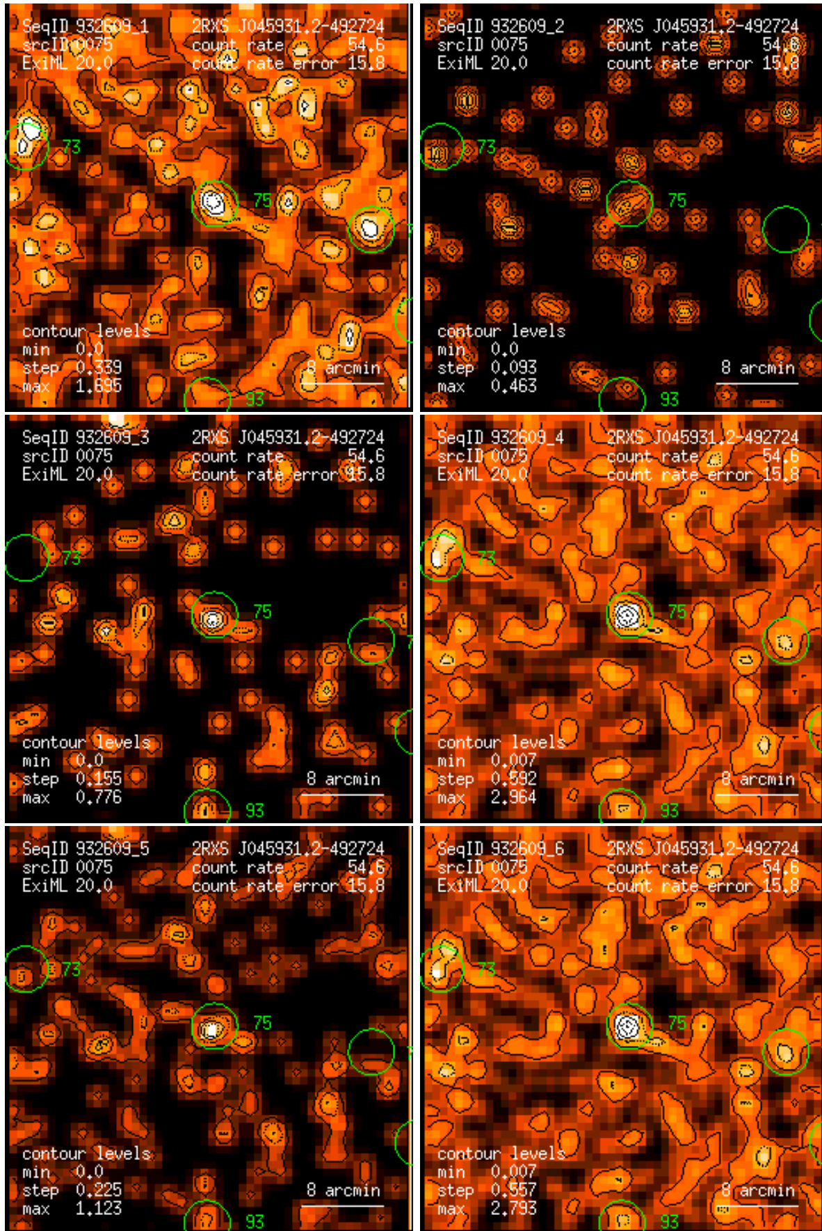
Figure 75: RASS 932609: detection 0075: band rate images, Gaussian filter: (1) PSPC channels 11 – 41, (2) 52 – 90, (3) 91 – 201, (4) 11 – 235, (5) 52 – 201, (6) 11 – 201. Broad band rates in counts/ks. Band rate contour levels in counts/ks/arcmin 2 .
