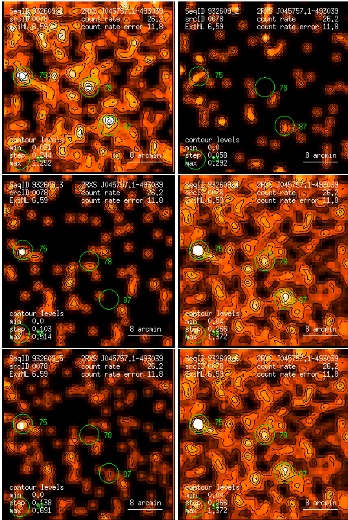
Figure 78: RASS 932609: detection 0078: band rate images, Gaussian filter: (1) PSPC channels 11 – 41, (2) 52 – 90, (3) 91 – 201, (4) 11 – 235, (5) 52 – 201, (6) 11 – 201. Broad band rates in counts/ks. Band rate contour levels in counts/ks/arcmin 2 .
