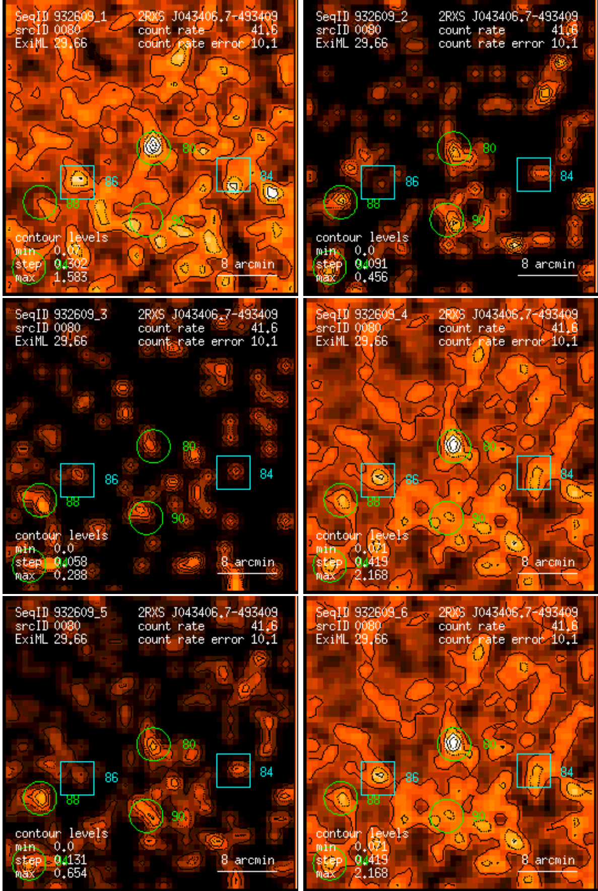
Figure 80: RASS 932609: detection 0080: band rate images, Gaussian filter: (1) PSPC channels 11 – 41, (2) 52 – 90, (3) 91 – 201, (4) 11 – 235, (5) 52 – 201, (6) 11 – 201. Broad band rates in counts/ks. Band rate contour levels in counts/ks/arcmin 2 .
