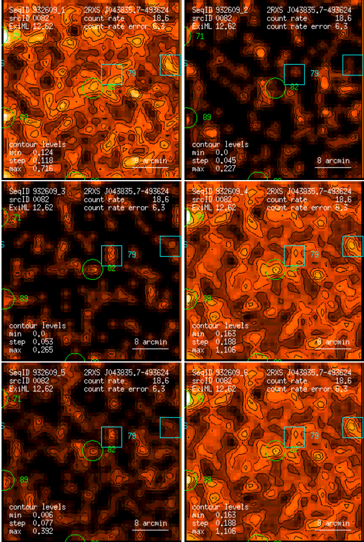
Figure 82: RASS 932609: detection 0082: band rate images, Gaussian filter: (1) PSPC channels 11 – 41, (2) 52 – 90, (3) 91 – 201, (4) 11 – 235, (5) 52 – 201, (6) 11 – 201. Broad band rates in counts/ks. Band rate contour levels in counts/ks/arcmin 2 .
