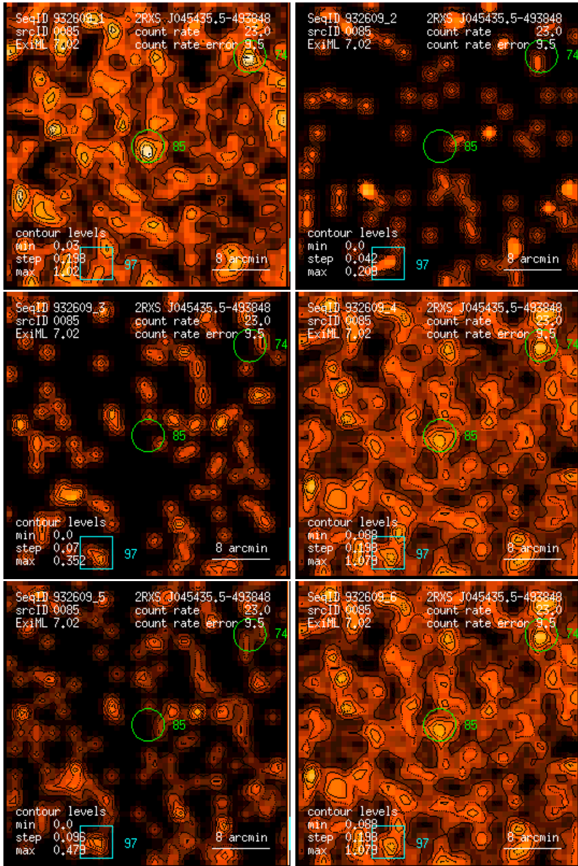
Figure 85: RASS 932609: detection 0085: band rate images, Gaussian filter: (1) PSPC channels 11 – 41, (2) 52 – 90, (3) 91 – 201, (4) 11 – 235, (5) 52 – 201, (6) 11 – 201. Broad band rates in counts/ks. Band rate contour levels in counts/ks/arcmin 2 .
