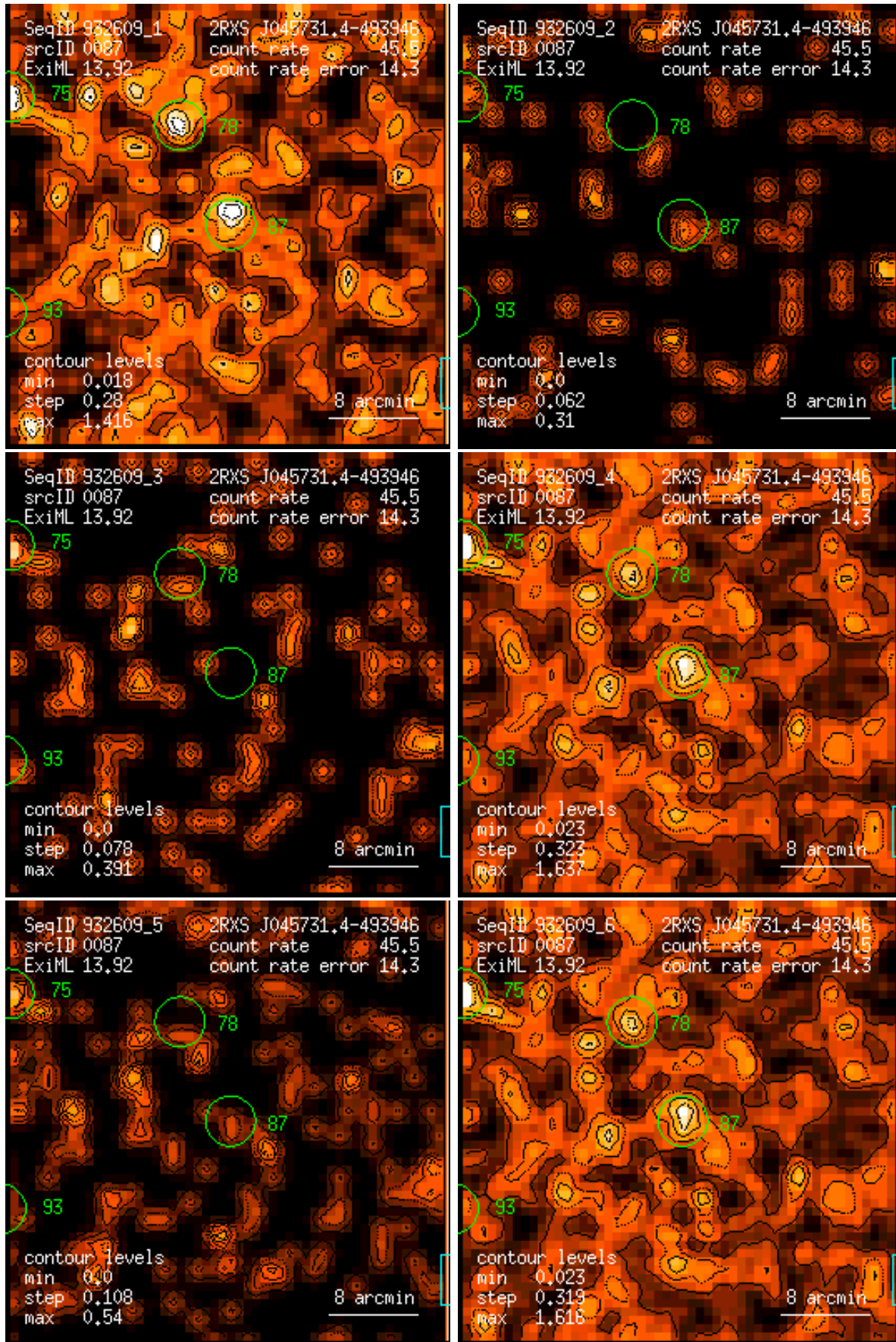
Figure 87: RASS 932609: detection 0087: band rate images, Gaussian filter: (1) PSPC channels 11 – 41, (2) 52 – 90, (3) 91 – 201, (4) 11 – 235, (5) 52 – 201, (6) 11 – 201. Broad band rates in counts/ks. Band rate contour levels in counts/ks/arcmin 2 .
