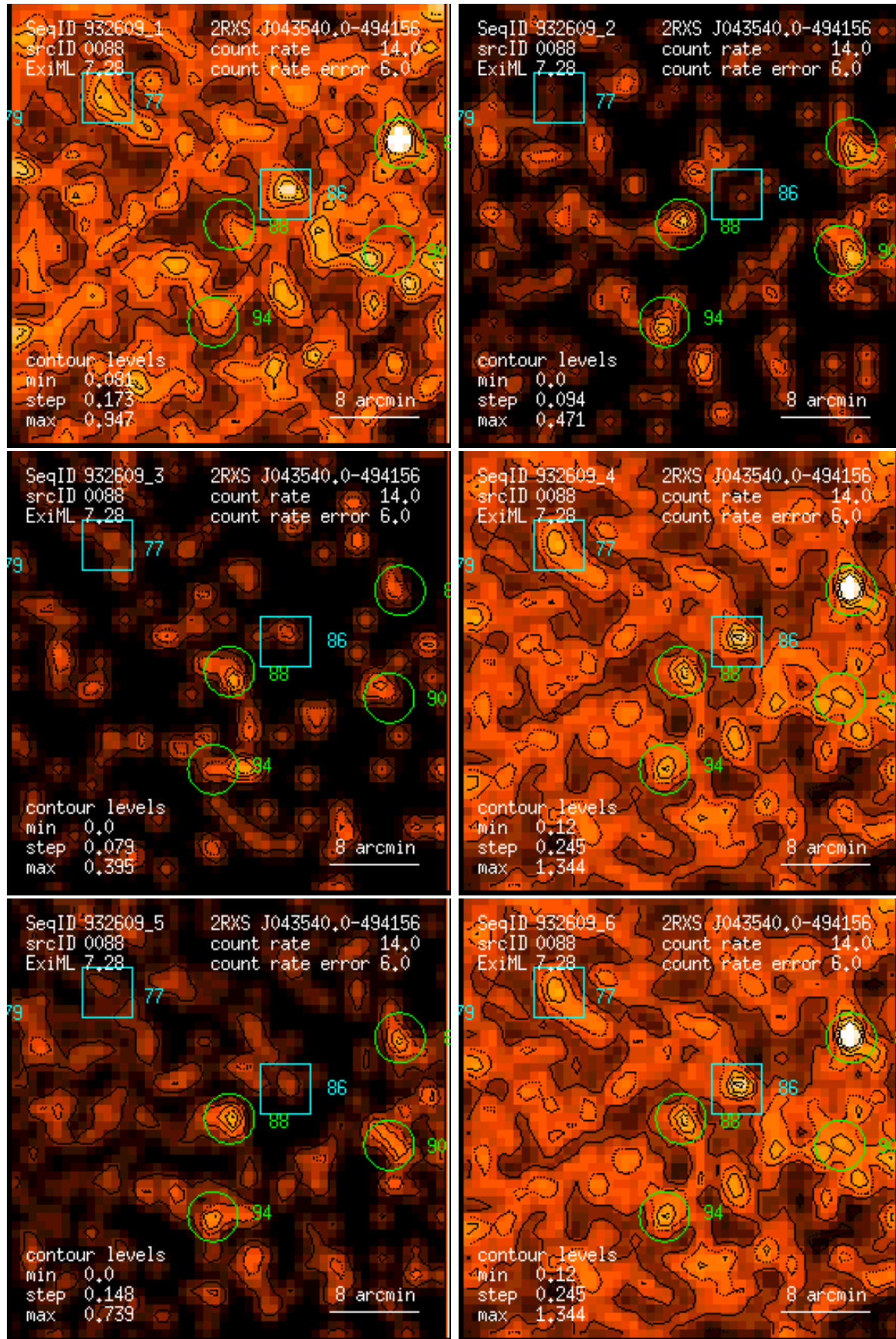
Figure 88: RASS 932609: detection 0088: band rate images, Gaussian filter: (1) PSPC channels 11 – 41, (2) 52 – 90, (3) 91 – 201, (4) 11 – 235, (5) 52 – 201, (6) 11 – 201. Broad band rates in counts/ks. Band rate contour levels in counts/ks/arcmin 2 .
