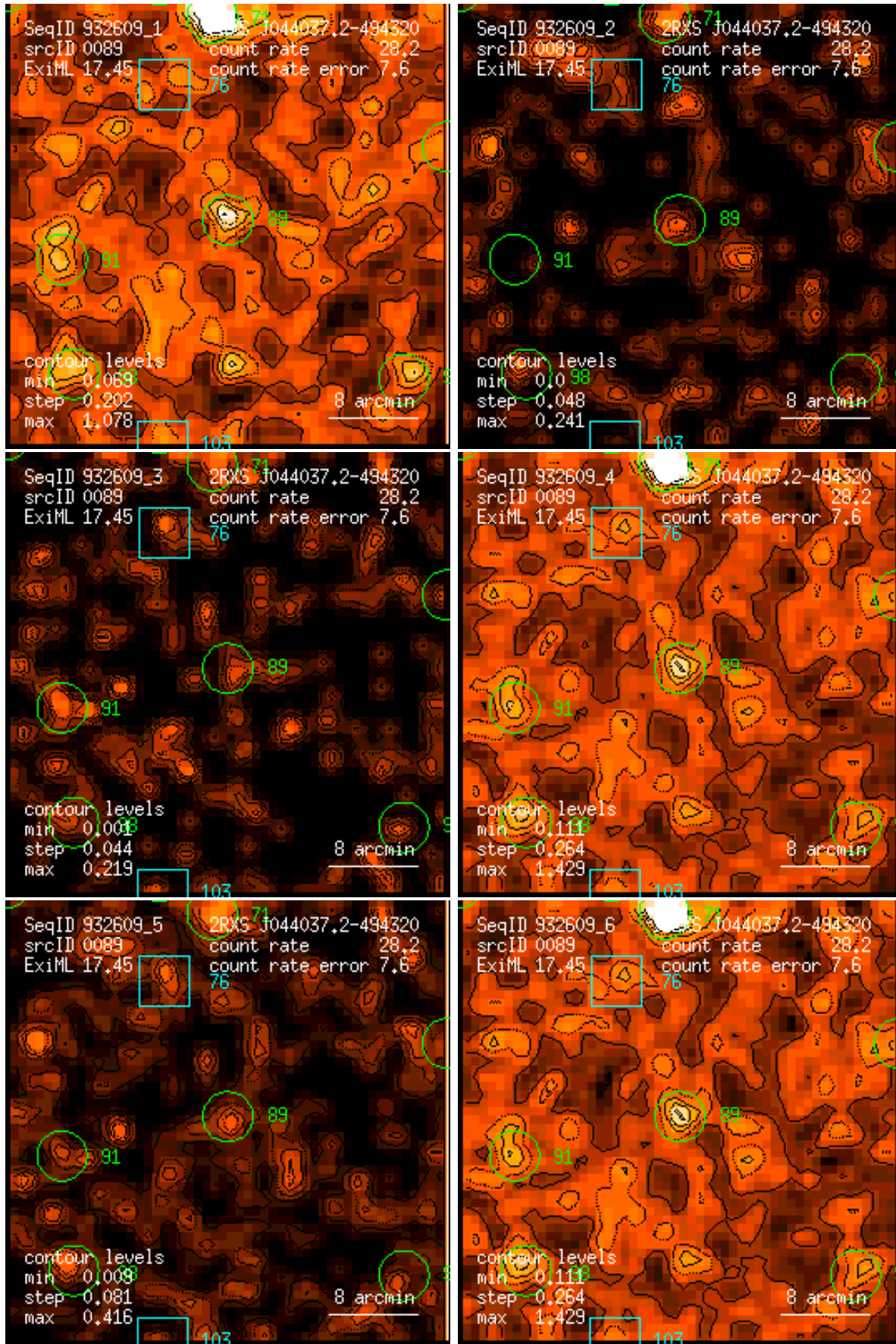
Figure 89: RASS 932609: detection 0089: band rate images, Gaussian filter: (1) PSPC channels 11 – 41, (2) 52 – 90, (3) 91 – 201, (4) 11 – 235, (5) 52 – 201, (6) 11 – 201. Broad band rates in counts/ks. Band rate contour levels in counts/ks/arcmin 2 .
