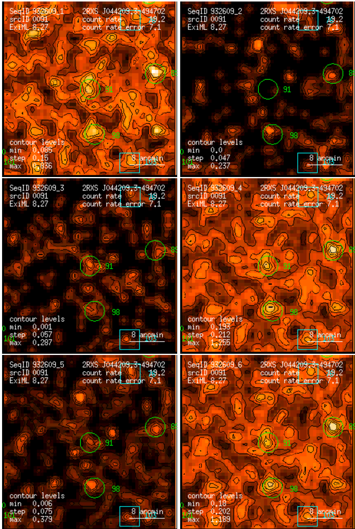
Figure 91: RASS 932609: detection 0091: band rate images, Gaussian filter: (1) PSPC channels 11 – 41, (2) 52 – 90, (3) 91 – 201, (4) 11 – 235, (5) 52 – 201, (6) 11 – 201. Broad band rates in counts/ks. Band rate contour levels in counts/ks/arcmin 2 .
