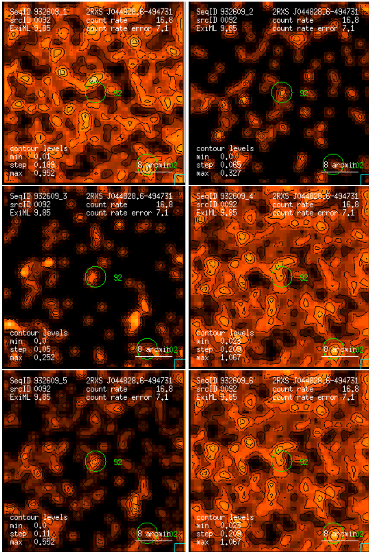
Figure 92: RASS 932609: detection 0092: band rate images, Gaussian filter: (1) PSPC channels 11 – 41, (2) 52 – 90, (3) 91 – 201, (4) 11 – 235, (5) 52 – 201, (6) 11 – 201. Broad band rates in counts/ks. Band rate contour levels in counts/ks/arcmin 2 .
