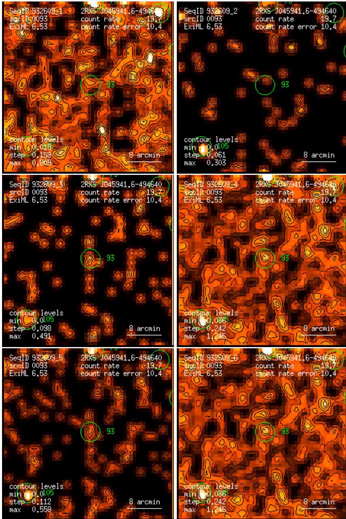
Figure 93: RASS 932609: detection 0093: band rate images, Gaussian filter: (1) PSPC channels 11 – 41, (2) 52 – 90, (3) 91 – 201, (4) 11 – 235, (5) 52 – 201, (6) 11 – 201. Broad band rates in counts/ks. Band rate contour levels in counts/ks/arcmin 2 .
