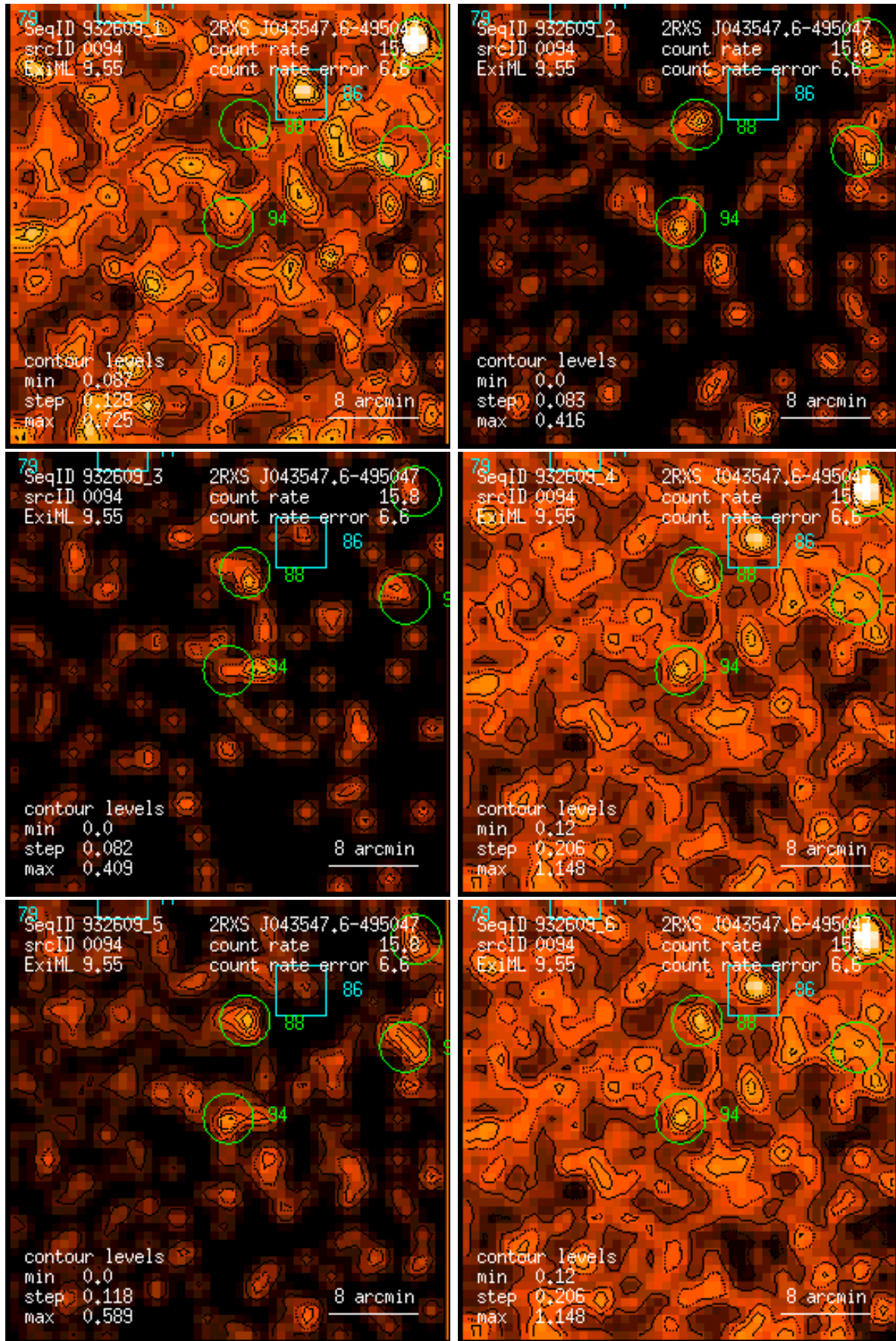
Figure 94: RASS 932609: detection 0094: band rate images, Gaussian filter: (1) PSPC channels 11 – 41, (2) 52 – 90, (3) 91 – 201, (4) 11 – 235, (5) 52 – 201, (6) 11 – 201. Broad band rates in counts/ks. Band rate contour levels in counts/ks/arcmin 2 .
