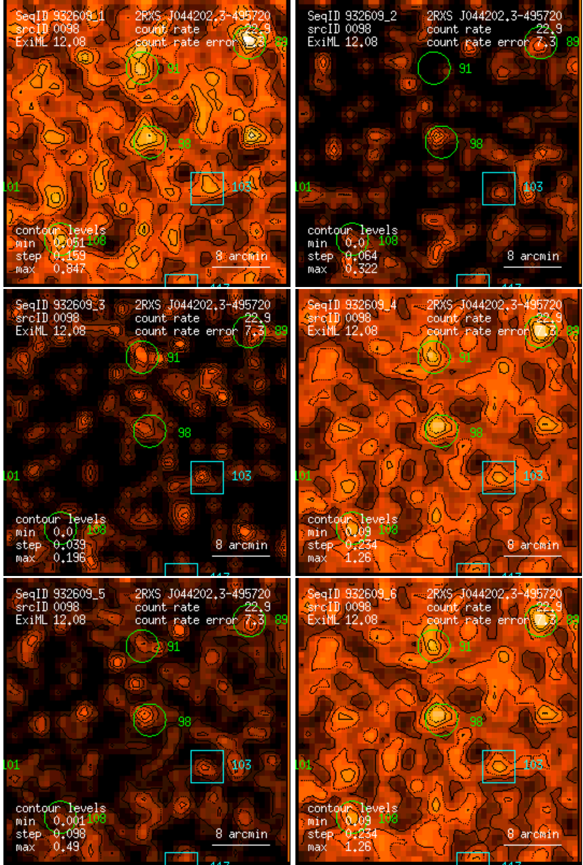
Figure 98: RASS 932609: detection 0098: band rate images, Gaussian filter: (1) PSPC channels 11 – 41, (2) 52 – 90, (3) 91 – 201, (4) 11 – 235, (5) 52 – 201, (6) 11 – 201. Broad band rates in counts/ks. Band rate contour levels in counts/ks/arcmin 2 .
