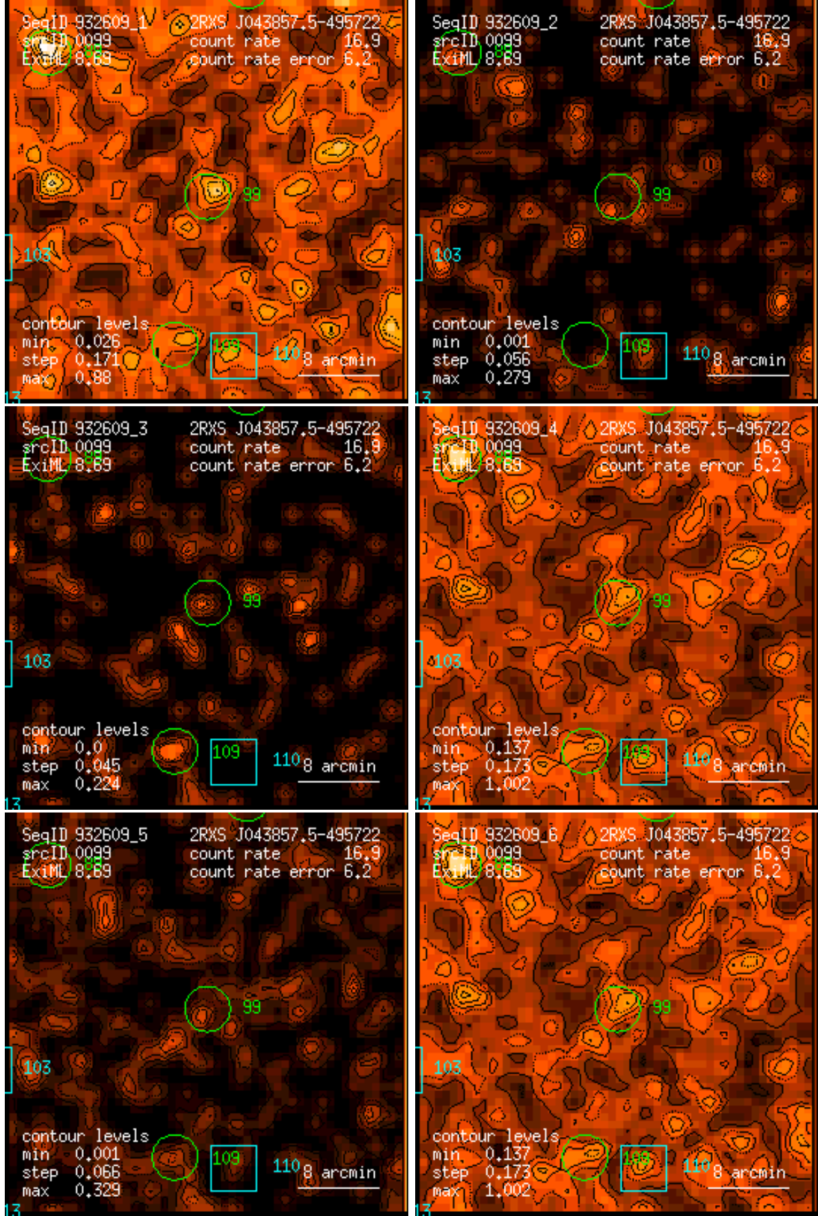
Figure 99: RASS 932609: detection 0099: band rate images, Gaussian filter: (1) PSPC channels 11 – 41, (2) 52 – 90, (3) 91 – 201, (4) 11 – 235, (5) 52 – 201, (6) 11 – 201. Broad band rates in counts/ks. Band rate contour levels in counts/ks/arcmin 2 .
