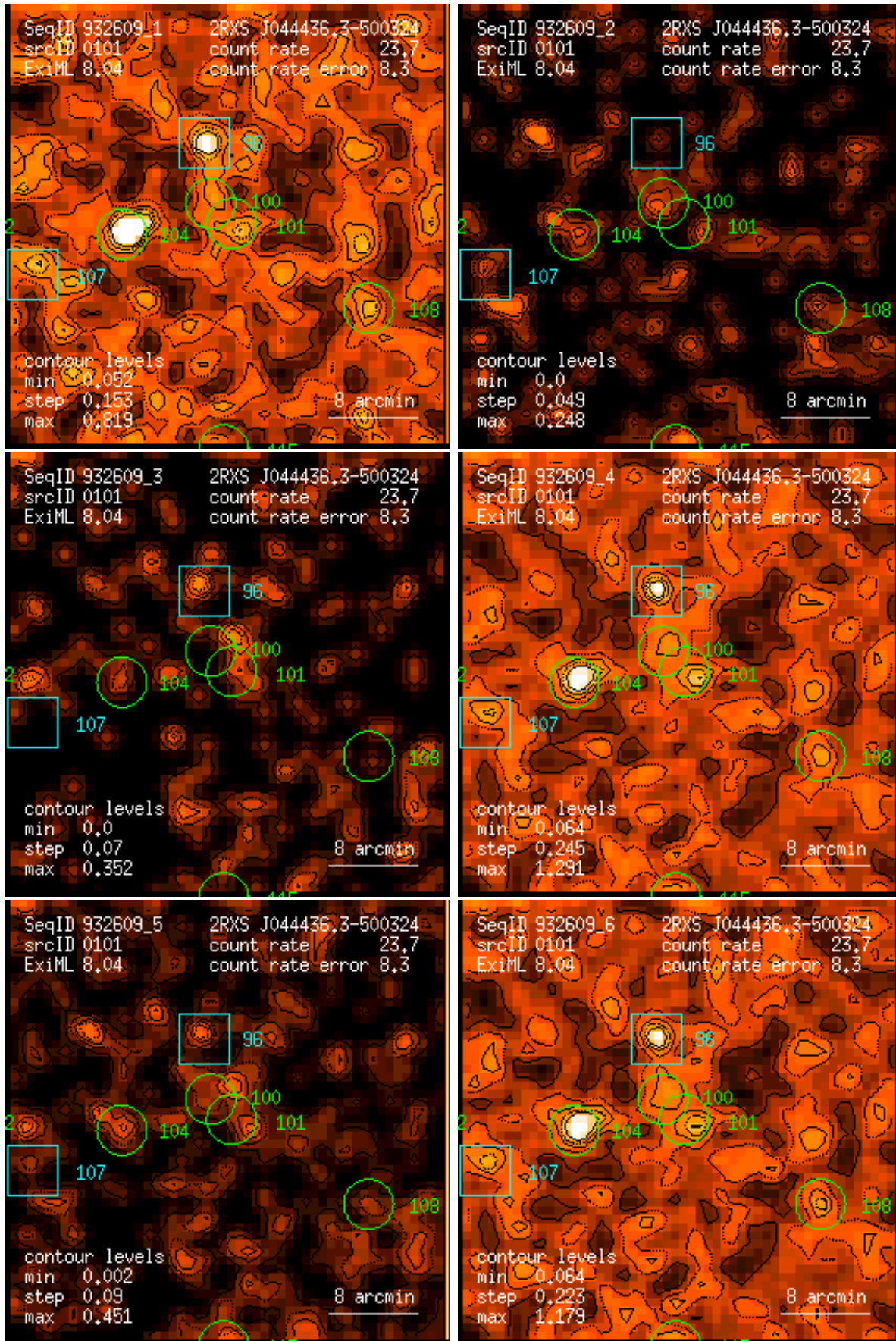
Figure 101: RASS 932609: detection 0101: band rate images, Gaussian filter: (1) PSPC channels 11 – 41, (2) 52 – 90, (3) 91 – 201, (4) 11 – 235, (5) 52 – 201, (6) 11 – 201. Broad band rates in counts/ks. Band rate contour levels in counts/ks/arcmin 2 .
