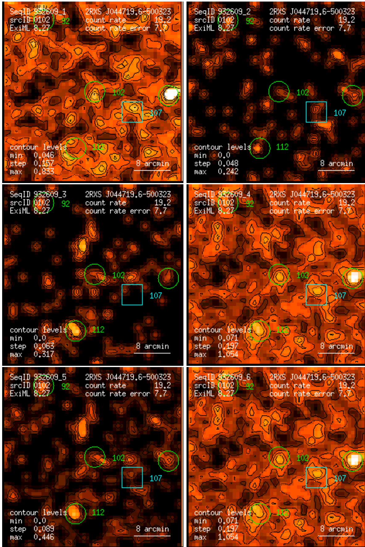
Figure 102: RASS 932609: detection 0102: band rate images, Gaussian filter: (1) PSPC channels 11 – 41, (2) 52 – 90, (3) 91 – 201, (4) 11 – 235, (5) 52 – 201, (6) 11 – 201. Broad band rates in counts/ks. Band rate contour levels in counts/ks/arcmin 2 .
