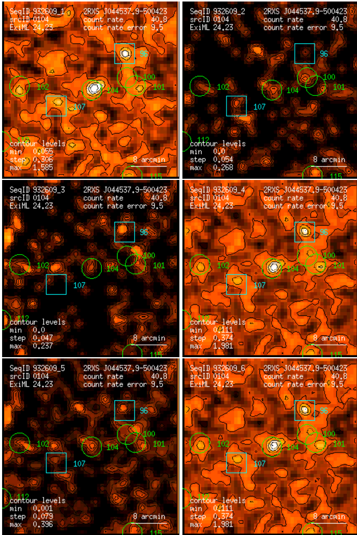
Figure 104: RASS 932609: detection 0104: band rate images, Gaussian filter: (1) PSPC channels 11 – 41, (2) 52 – 90, (3) 91 – 201, (4) 11 – 235, (5) 52 – 201, (6) 11 – 201. Broad band rates in counts/ks. Band rate contour levels in counts/ks/arcmin 2 .
