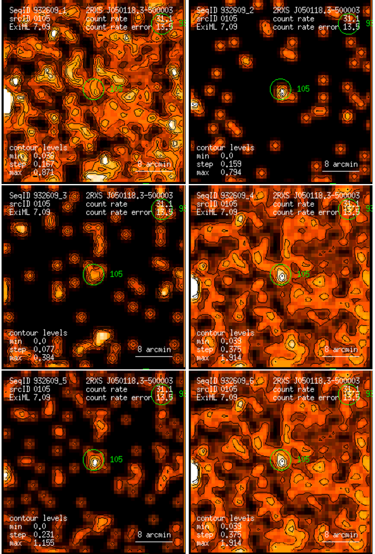
Figure 105: RASS 932609: detection 0105: band rate images, Gaussian filter: (1) PSPC channels 11 – 41, (2) 52 – 90, (3) 91 – 201, (4) 11 – 235, (5) 52 – 201, (6) 11 – 201. Broad band rates in counts/ks. Band rate contour levels in counts/ks/arcmin 2 .
