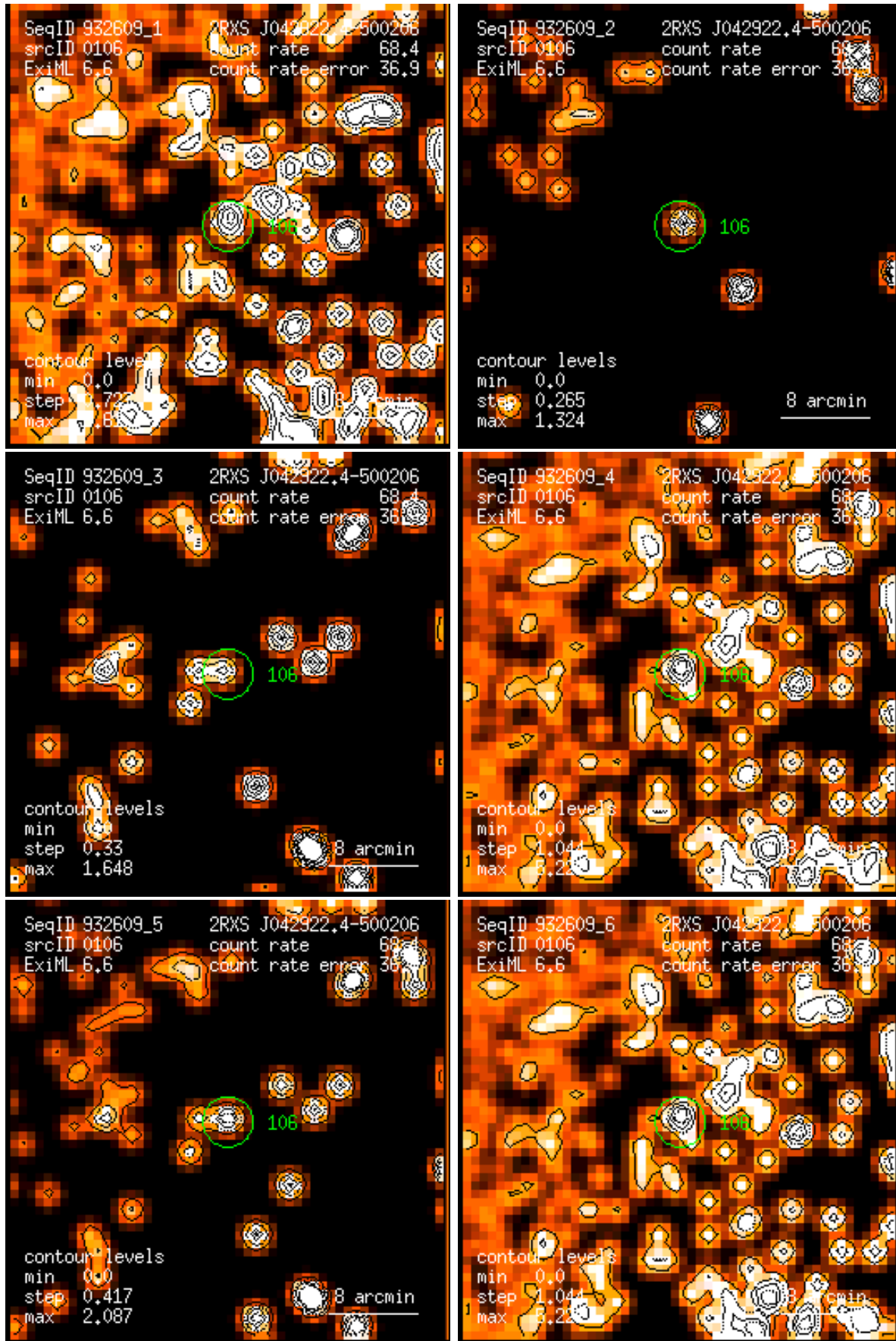
Figure 106: RASS 932609: detection 0106: band rate images, Gaussian filter: (1) PSPC channels 11 – 41, (2) 52 – 90, (3) 91 – 201, (4) 11 – 235, (5) 52 – 201, (6) 11 – 201. Broad band rates in counts/ks. Band rate contour levels in counts/ks/arcmin 2 .
