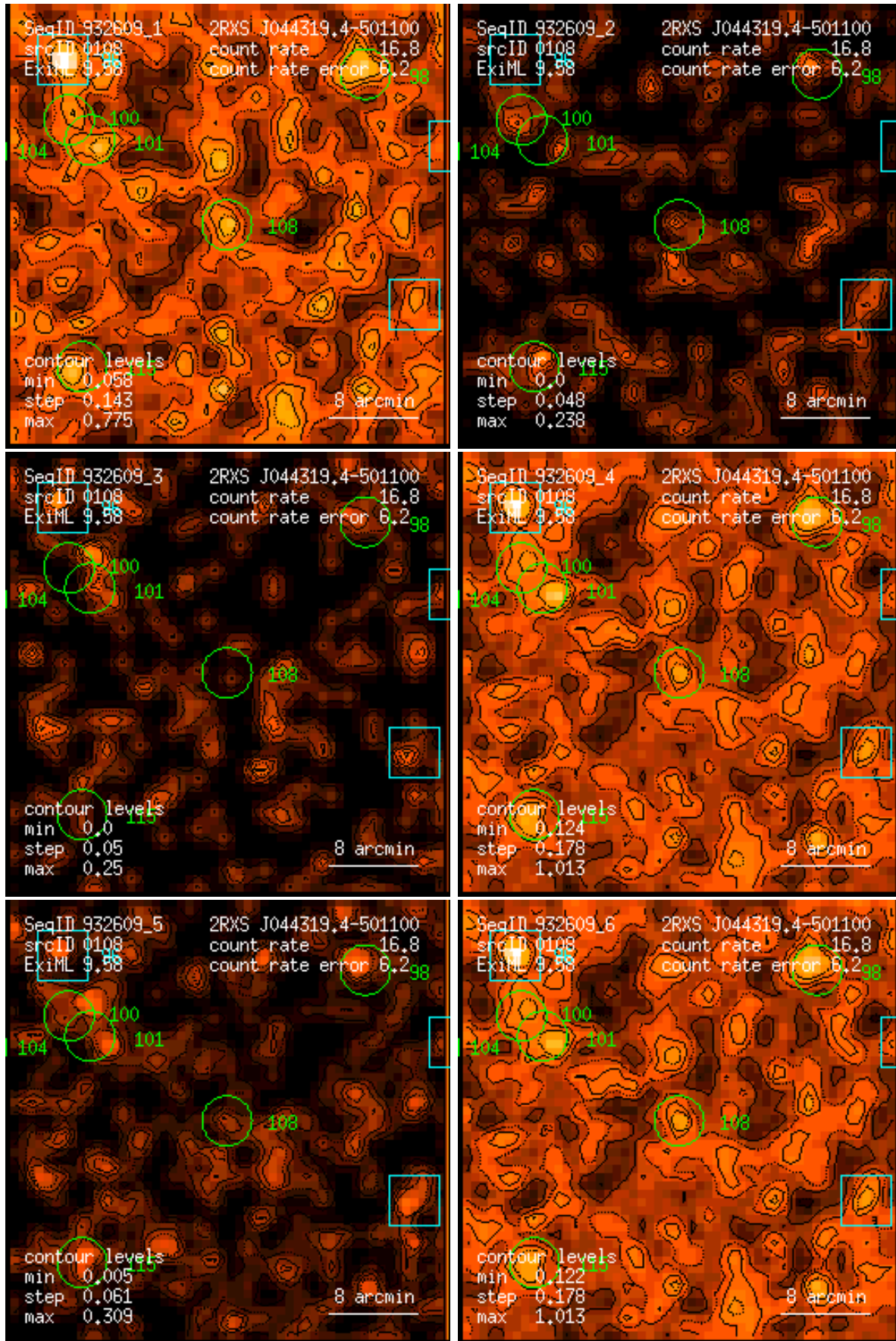
Figure 108: RASS 932609: detection 0108: band rate images, Gaussian filter: (1) PSPC channels 11 – 41, (2) 52 – 90, (3) 91 – 201, (4) 11 – 235, (5) 52 – 201, (6) 11 – 201. Broad band rates in counts/ks. Band rate contour levels in counts/ks/arcmin 2 .
