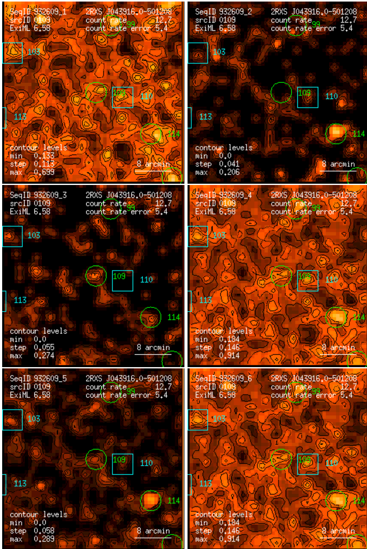
Figure 109: RASS 932609: detection 0109: band rate images, Gaussian filter: (1) PSPC channels 11 – 41, (2) 52 – 90, (3) 91 – 201, (4) 11 – 235, (5) 52 – 201, (6) 11 – 201. Broad band rates in counts/ks. Band rate contour levels in counts/ks/arcmin 2 .
