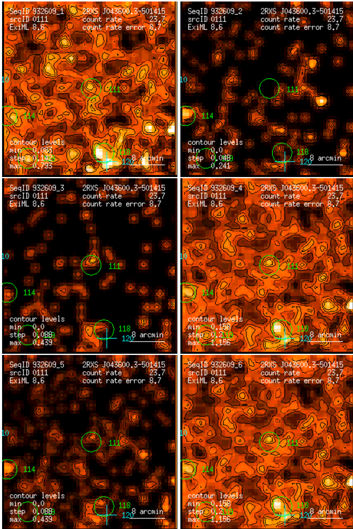
Figure 111: RASS 932609: detection 0111: band rate images, Gaussian filter: (1) PSPC channels 11 – 41, (2) 52 – 90, (3) 91 – 201, (4) 11 – 235, (5) 52 – 201, (6) 11 – 201. Broad band rates in counts/ks. Band rate contour levels in counts/ks/arcmin 2 .
