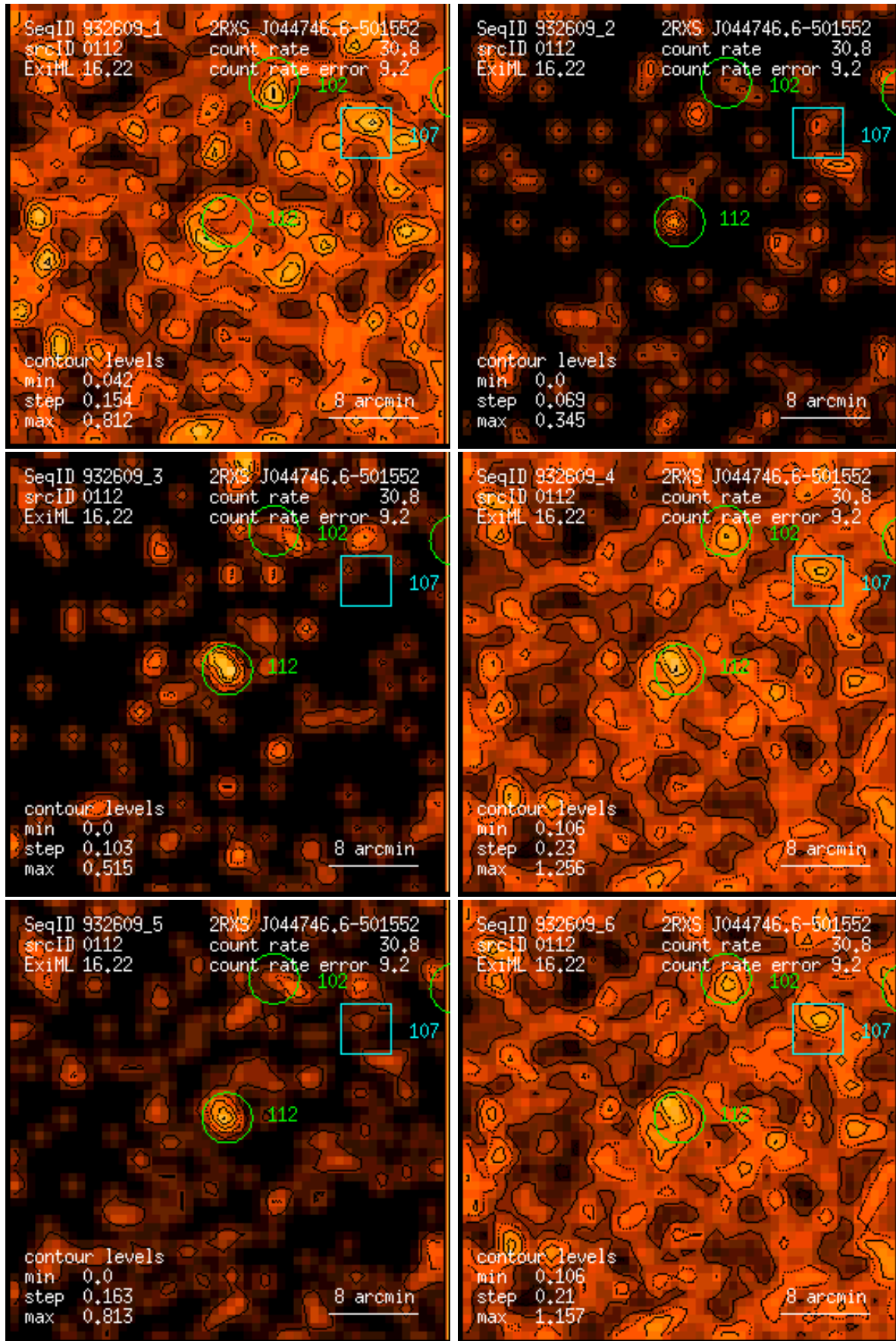
Figure 112: RASS 932609: detection 0112: band rate images, Gaussian filter: (1) PSPC channels 11 – 41, (2) 52 – 90, (3) 91 – 201, (4) 11 – 235, (5) 52 – 201, (6) 11 – 201. Broad band rates in counts/ks. Band rate contour levels in counts/ks/arcmin 2 .
